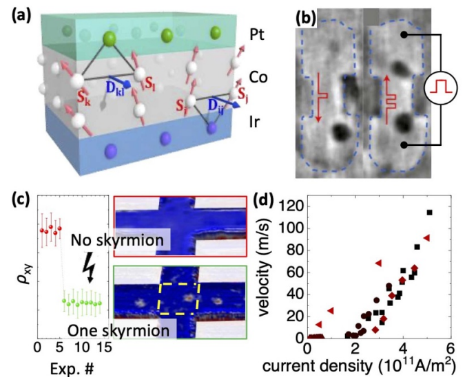
Figure 15. (a) Unit cell of a (\text{Ir}/\text{Co}/\text{Pt}) \times 20 multilayer with additive DMI at the interfaces of a 0.6-nm-thick Co layers with Ir and Pt. The thin Ir and Pt layers couple the skyrmions in the different layers in a single column of skyrmions [149]. (b) Creation of skyrmions at the edge of a constriction in a (\text{Pt}/\text{CoFeB}/\text{MgO}) \times 15 multilayer by successive current pulses in opposite directions (track width is 400 nm) [152]. (c) Detection of the presence of a single skyrmion by the change in AHE ( 25 \text{ n}\Omega \text{ cm} in this specific example using the multilayer of (a)) [154]. (d) Skyrmion velocity as a function of the current density in different types of multilayers (from recent literature). (a) Reprinted by permission from Springer Nature Customer Service Centre GmbH: Nature Nanotechnology [149] Copyright (2016). (b) Reprinted by permission from Springer Nature Customer Service Centre GmbH: Nature Nanotechnology [152] Copyright (2017). (c) Reprinted by permission from Springer Nature Customer Service Centre GmbH: Nature Nanotechnology [154] Copyright (2018).
