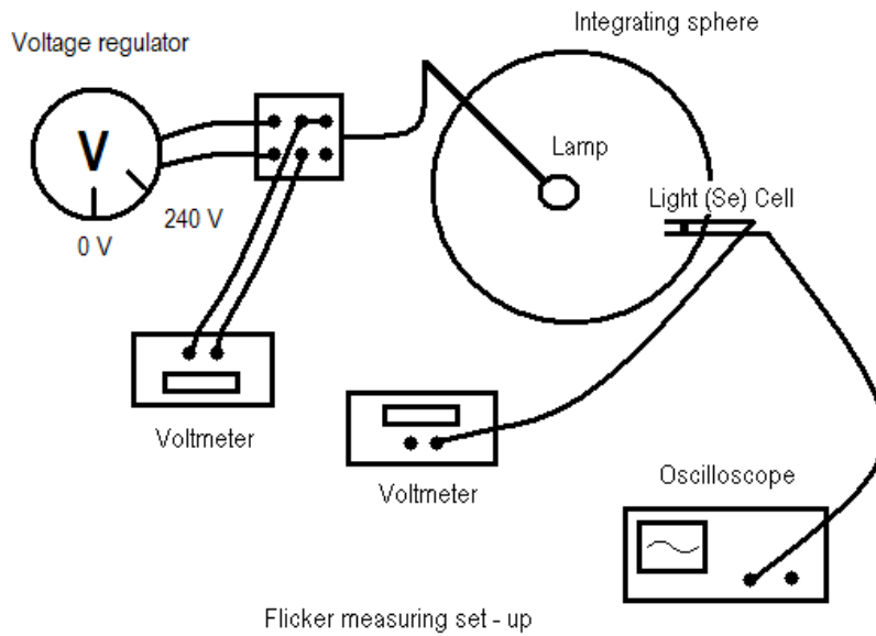
Figure 1. Diagram of the measuring set up
