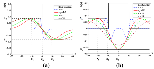
Fig. 3 LoG responses at different scales to a step function b a boxcar function of size w = 21
