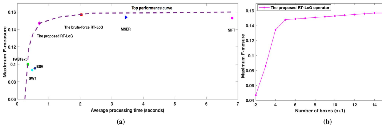
Fig. 20 a Comparison of operators with the maximum F-measure scores against the average processing time b the maximum F-measure score corresponding to the number of boxes for the proposed RT-LoG operator on ICDAR2017 RRC-MLT dataset
