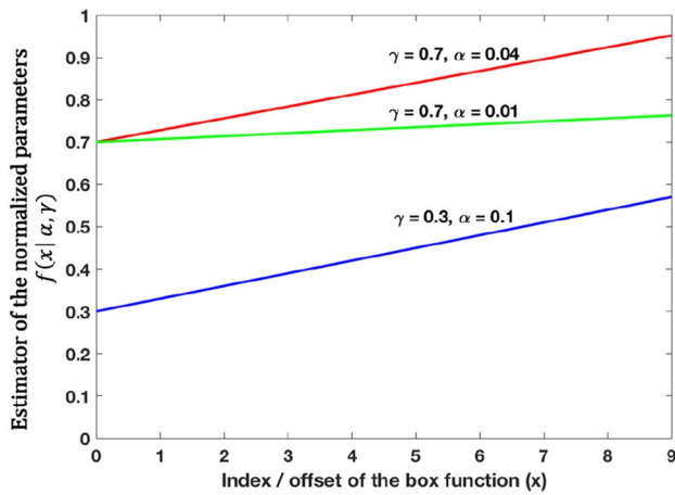
Fig. 13 The function f(x|\alpha, \gamma) for spatial/scale-space selection
