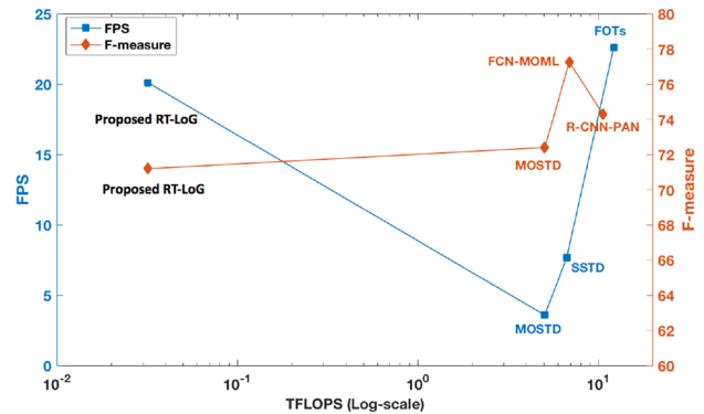
Fig. 22 The details of F-measure scores and FPS from scene text detection systems correspond to their architectures
