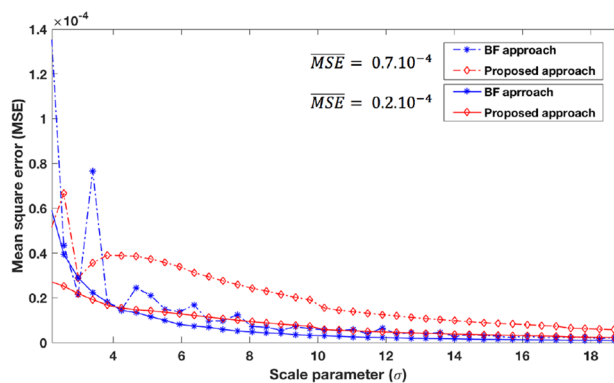
Fig. 15 DoG approximation of the operators over scales at the equal \overline{MSE}
