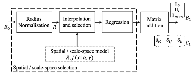
Fig. 12 Spatial/scale-space selection
