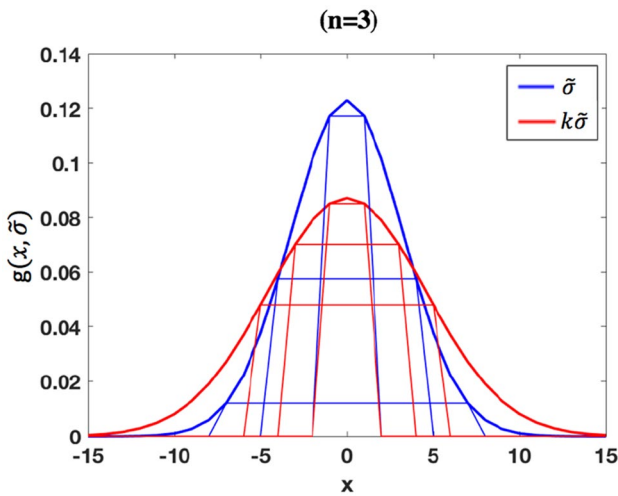
Fig. 8 The box functions to approximate two Gaussian kernels k\tilde{\sigma} and \tilde{\sigma} with \tilde{\sigma} = 3.2 and k = \sqrt{2}
