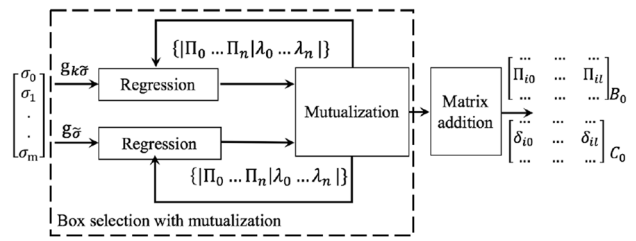
Fig. 9 Box selection with mutualization for the \widehat{DoG}
