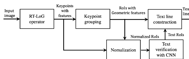
Fig. 21 The general architecture of the system of [32]
