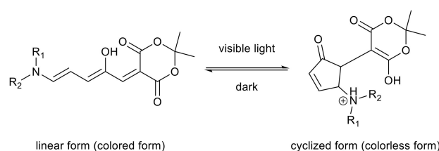
Scheme 1. General structures of the open/closed forms of the Donor–acceptor Stenhouse adducts (DASA) based on Meldrum’s acid.
