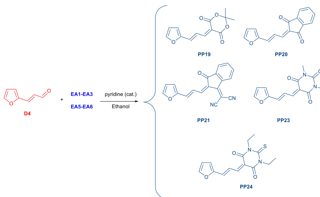
Scheme 2. Synthetic route to PP1–PP5 , PP7–PP9 , PP13–PP21 , PP23–PP24 .
