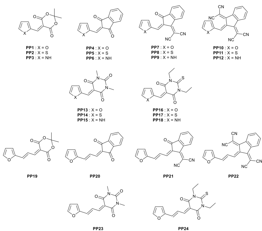
Figure 1. Chemical structures of PP1–PP24 used as precursors for the design of Donor–acceptor Stenhouse adducts (DASA) photoswitches.
