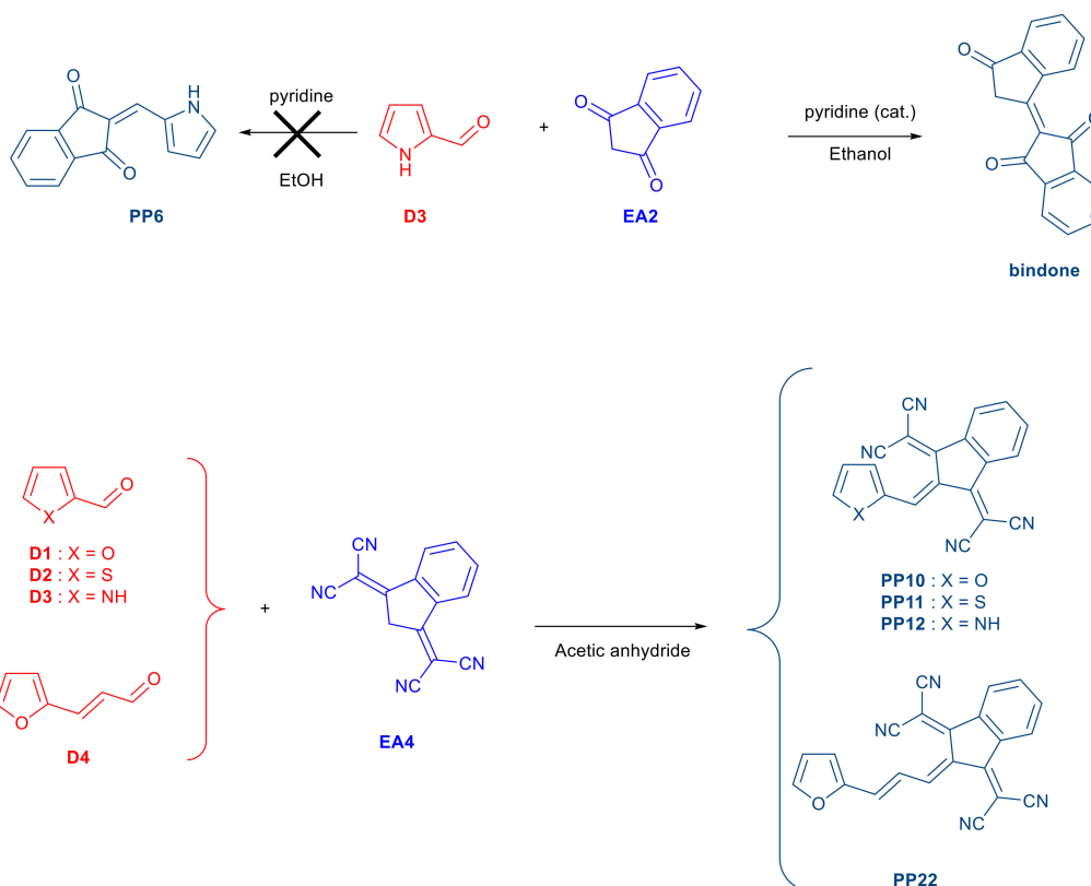
Scheme 3. Synthetic route to PP10–PP12 and PP22 .
