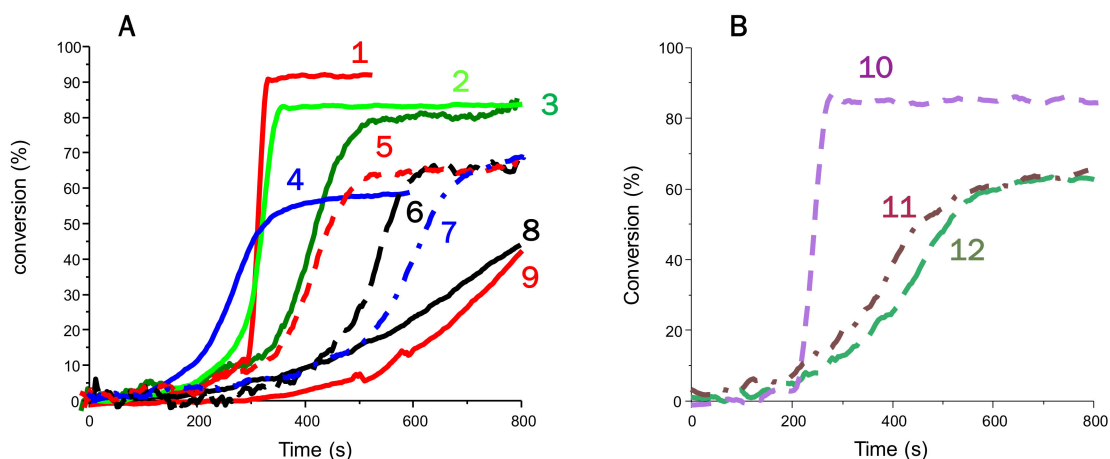
Figure 9. Real Time Fourier Transform Infrared (RT-FTIR) photopolymerization kinetics (C=C conversion vs. irradiation time; 1.4 mm thick sample) under air upon exposure to a Laser Diode@785nm; 2.5 W/cm 2 ; for Mix-MA in the presence of dye/iodonium/4-dppba/BlocBuilder MA(0.1/2/2/2% w/w); the irradiation starts after 15 s for: (A) (1) DASA1; (2) DASA2; (3) DASA3; (4) DASA4; (5) DASA5; (6) DASA12; (7) DASA10; (8) DASA9; (9) DASA11; (B) (10) DASA7; (11) PP25; (12) PP26.
