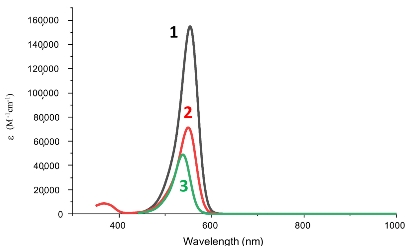
Figure 6. UV-vis absorption spectra of DASA12 (1); DASA11 (2) and DASA9 (3) in acetonitrile.
