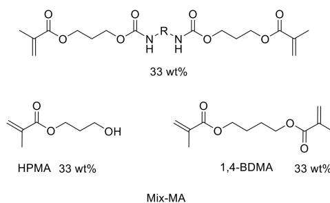
Figure 5. Benchmark methacrylate monomer blend Mix-MA.
