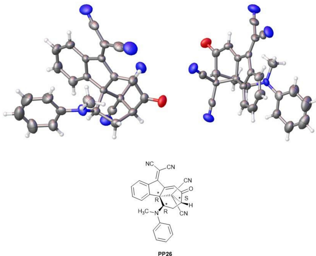
Figure 4. Crystal structure of PP26.
