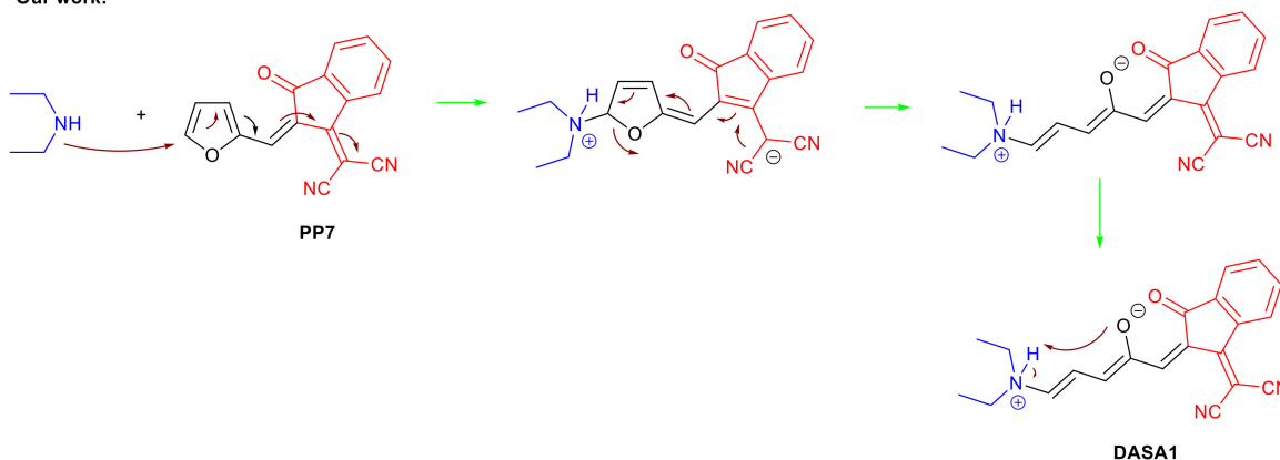
Scheme 6. Mechanisms involved in the synthesis of cyclization product (CP1) and DASA1.
