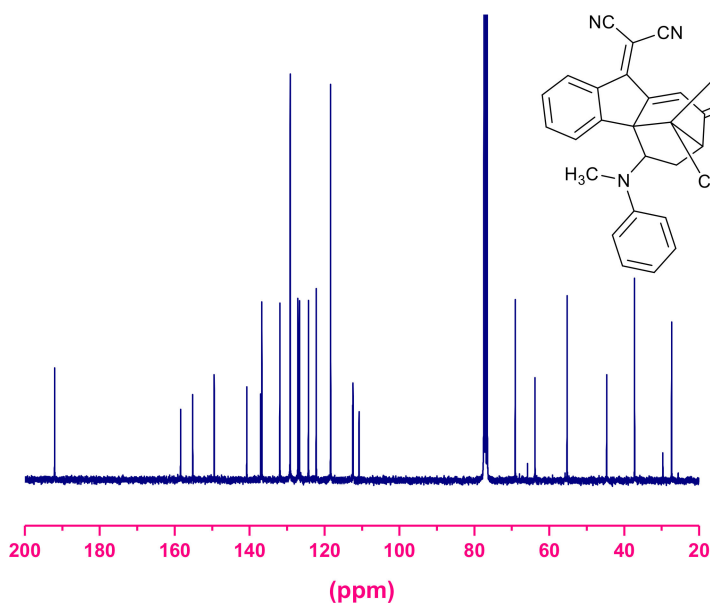
Figure 3. Proton nuclear magnetic resonance ( ^1\text{H-NMR} ) spectrum (a) and carbon-13 nuclear magnetic resonance ( ^{13}\text{C NMR} ) spectrum (b) of cyclized compound PP26 .
