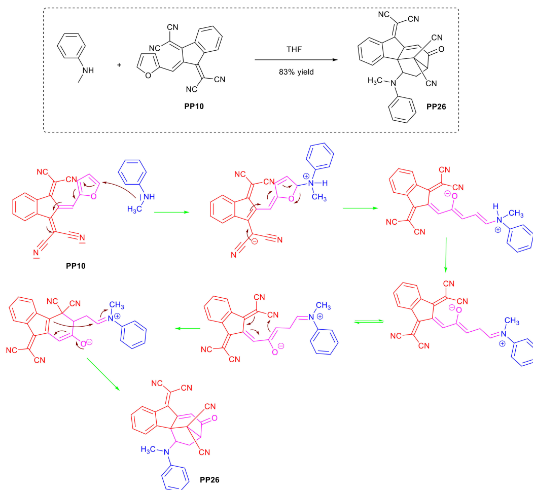
Scheme 7. Mechanisms supporting the formation of PP26 .
