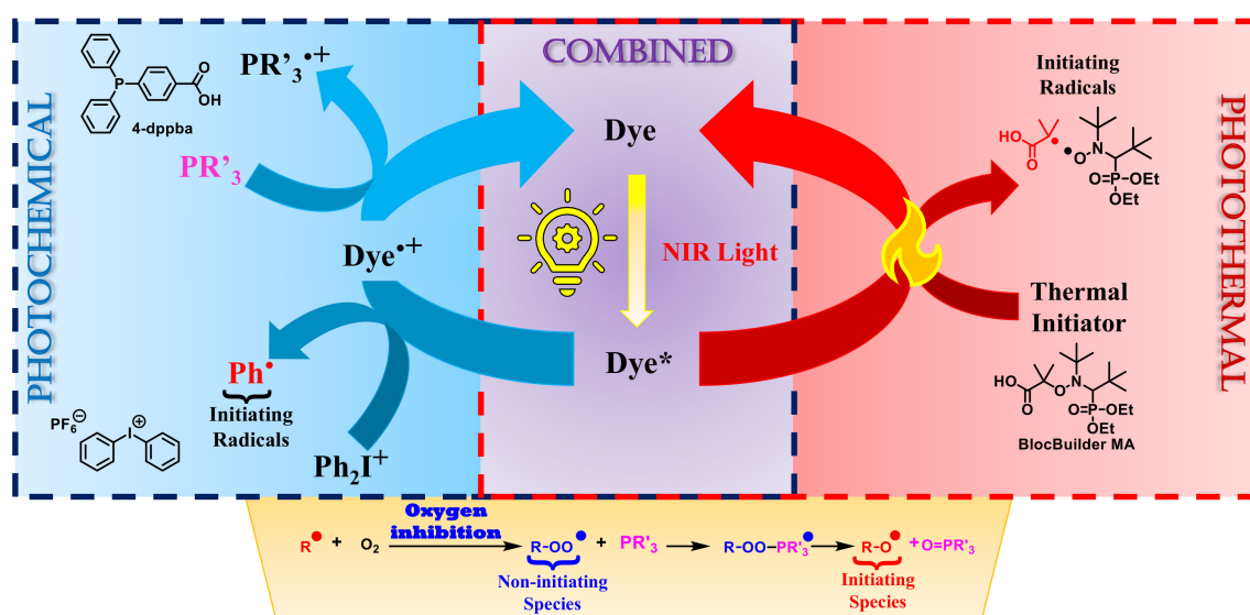
Figure 8. Overview of the chemical mechanism.
