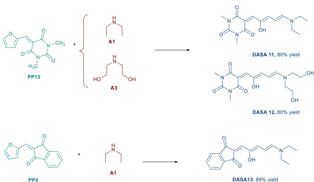
Scheme 5. Synthetic route to DASA10–DASA13.
