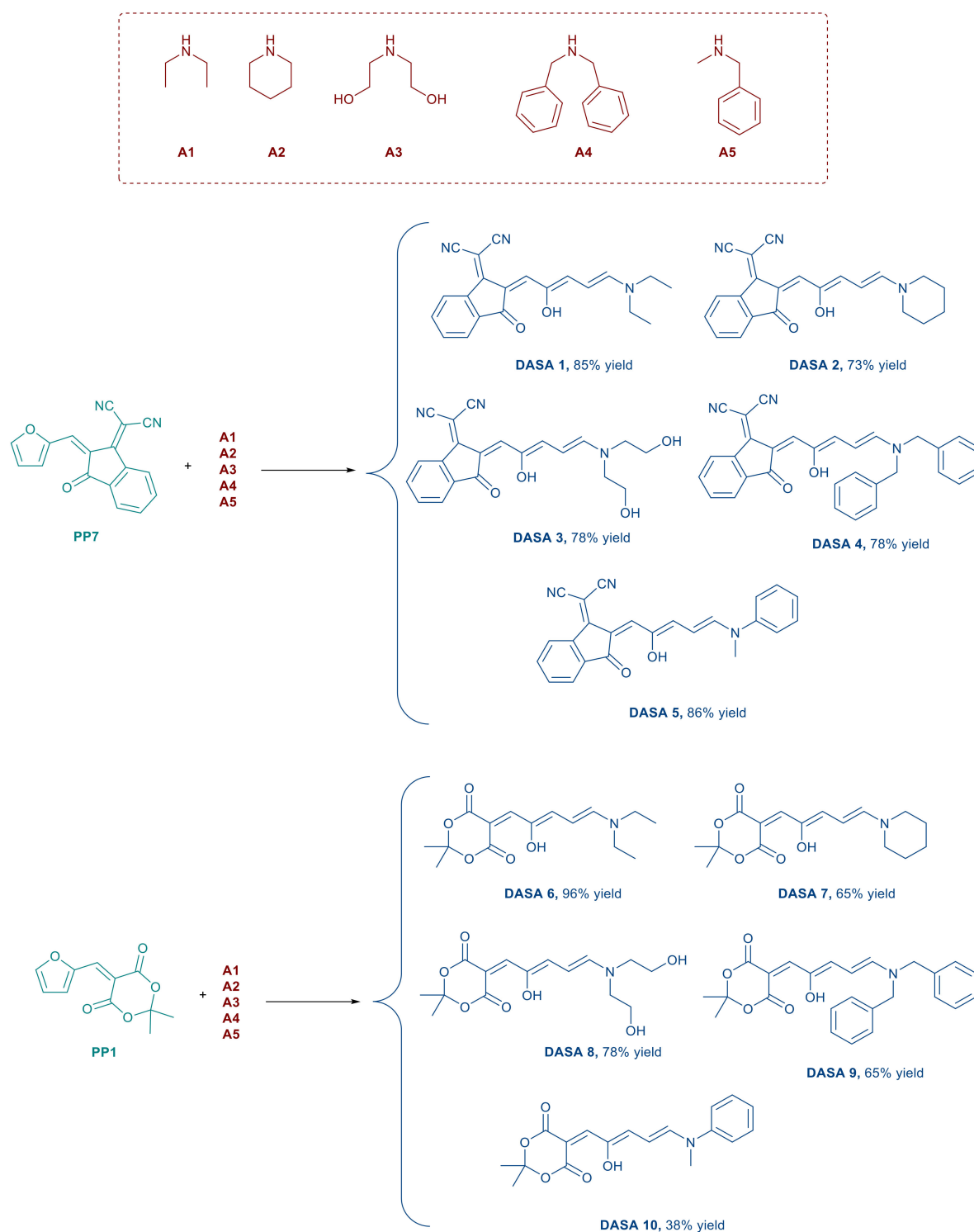
Scheme 4. Synthetic route to DASA1–DASA10. Investigated amines were: diethylamine (A1), piperidine (A2), diethanolamine (A3), dibenzylamine (A4) and N -methylbenzylamine (A5).
