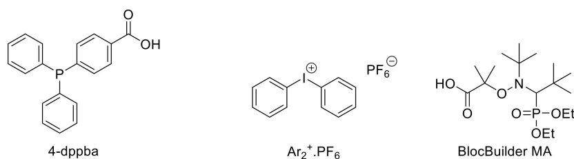
Figure 7. Chemical structures of additives.
