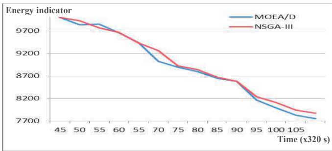
Fig. 7. Variation of energy in relation to the number of fixed nodes, for 4 objectives
