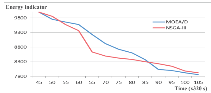
Fig. 6. Variation of energy in relation to the number of fixed nodes, for 2 objectives
