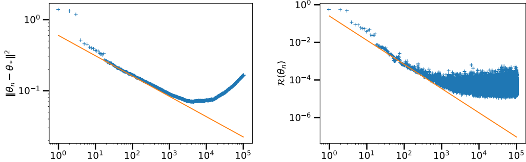
Figure 4: In blue +, evolution of \|\theta_n - \theta_*\|^2 (left) and \mathcal{R}(\theta_n) (right) as functions of n , for the problems with parameters d = 10^5, \beta = 1.4, \delta = 1.2 . The orange lines represent the curves D/n^{\alpha_*} (left) and D'/n^{\alpha_*+1} (right).
