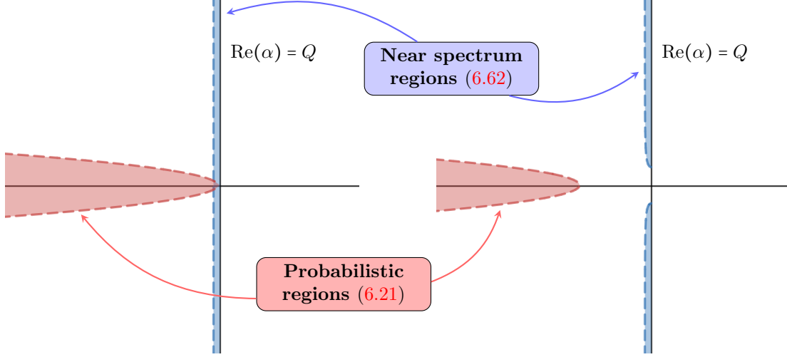
FIGURE 3. Left picture: regions of definition of the Poisson operator \mathcal{P}_0(\alpha) (for the plot, we take \gamma = 1/2 and \beta_0 is optimized to obtain the largest possible region). Right picture: regions of definition of the Poisson operator \mathcal{P}_\ell(\alpha) with \ell > 0 (for the plot we take \lambda_\ell = 4, \gamma = 1/2 and \beta_\ell optimized).
