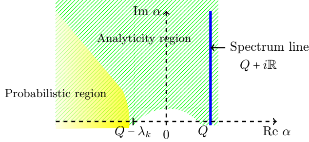
FIGURE 1. Analytic continuation of eigenstates and probabilistic region.
