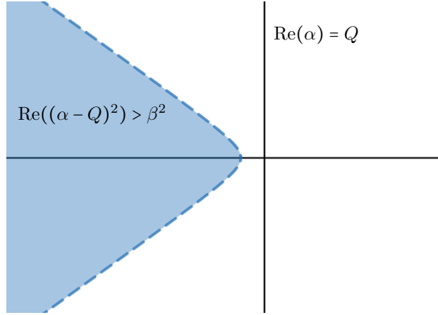
FIGURE 2. The blue region corresponds to the set of parameters \alpha \in \mathbb{C} such that \operatorname{Re}((\alpha - Q)^2) > \beta^2 , i.e. region of validity of Lemma 6.5 (here \beta = 1 on the plot).
