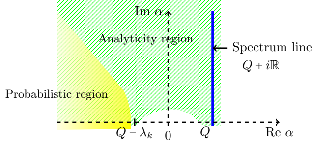
FIGURE 1. Analytic continuation of eigenstates and probabilistic region.
