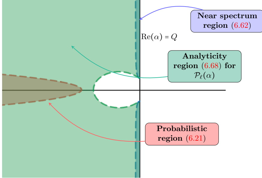
FIGURE 4. The green colored region correspond to the region (6.68) of validity of Lemma 6.21 for the analyticity of the Poisson operator \mathcal{P}_\ell(\alpha) with \ell > 0 (for the plot, we take \lambda_\ell = 4 , \gamma = 1/2 ). It overlaps the probabilistic (6.21) and near spectrum (6.62) regions.
