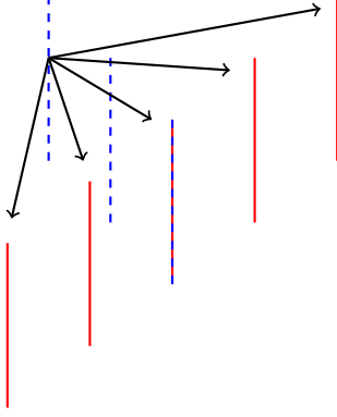
FIGURE 1. Schematic picture of the band structure. The dashed blue lines represent the bands \sigma_0^0, \sigma_0^1, \sigma_0^2 . The red solid lines represent the bands \sigma_{-2}^0, \sigma_{-1}^0, \sigma_0^0, \sigma_1^0, \sigma_2^0 . The arrows illustrate that the operators J_{0,\lambda}^3 from Corollary A.9 relate \sigma_0^2 and \bigcup_{a+b=2} \sigma_{a-b}^0 .
