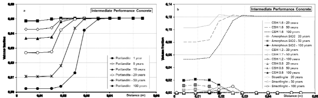
Fig. 7. Evolution of volume fraction for portlandite (a) and CSH phases and amorphous silica (b) for the Intermediate Performance Concrete (calculated with the EOS4 module using liquid saturation effect).
