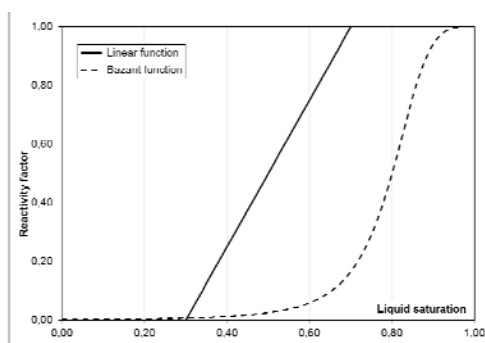
Fig. 6. Chemical reactivity factor as a function of the liquid saturation.
