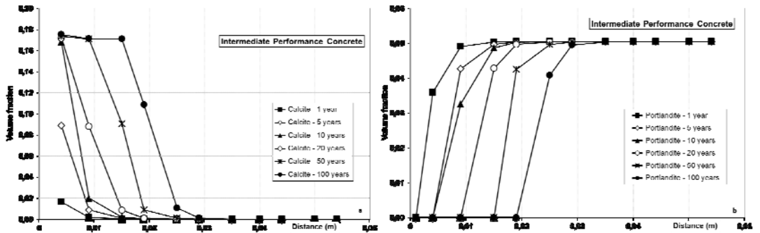
Fig. 4. Evolution of volume fraction profiles for calcite (a) and portlandite (b) for the Intermediate Performance Concrete (calculated with the EOS4 module).
