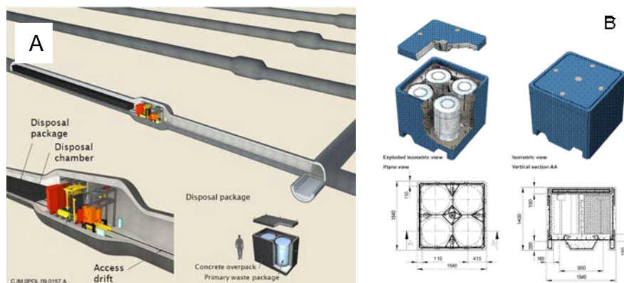
Fig. 1. Concrete components – A: view of the ILLW disposal cell – B: view of the ILLW disposal package.
