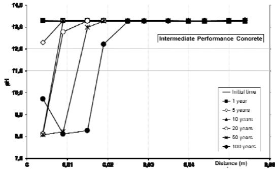
Fig. 3. Evolution of pH profiles for the Intermediate Performance Concrete (calculated with the EOS4 module).
