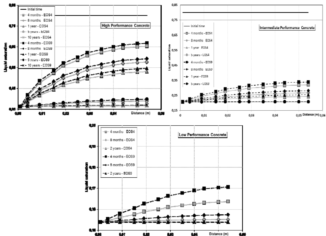
Fig. 2. Evolution of the liquid saturation profiles with time for the three concrete materials.
