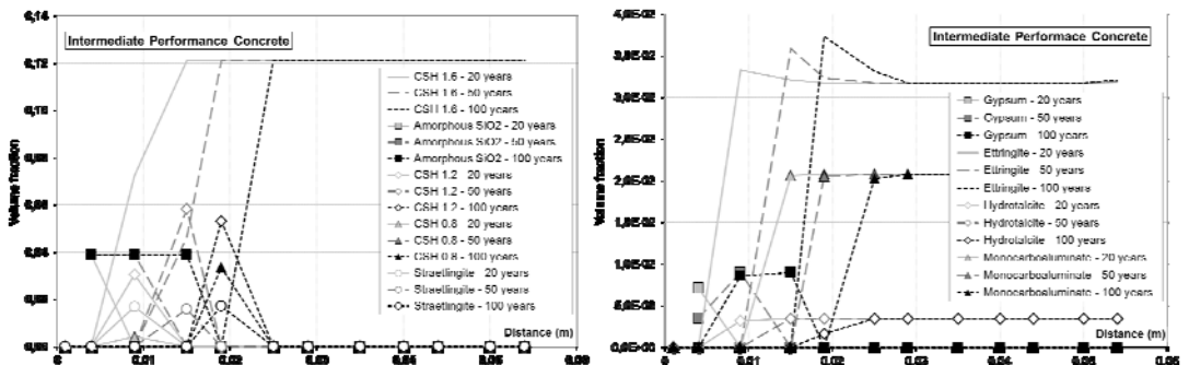
Fig. 5. Evolution of volume fraction profiles for CSH phases and amorphous silica (a) and selected accessory phases (b) for the Intermediate Performance Concrete (calculated with the EOS4 module)
