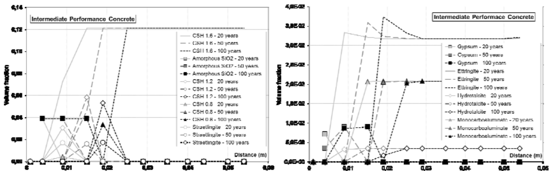
Fig. 5. Evolution of volume fraction profiles for CSH phases and amorphous silica (a) and selected accessory phases (b) for the Intermediate Performance Concrete (calculated with the EOS4 module)
