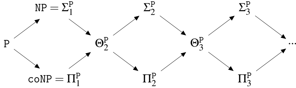
Figure 3.1: Polynomial hierarchy
