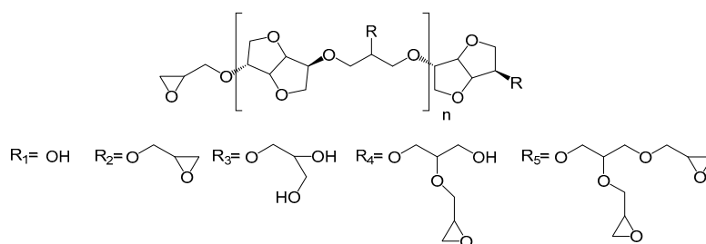
Scheme 2. Structures of the oligo-isosorbide glycidyl ethers [\text{R}_x]_n\text{-R}_x .
