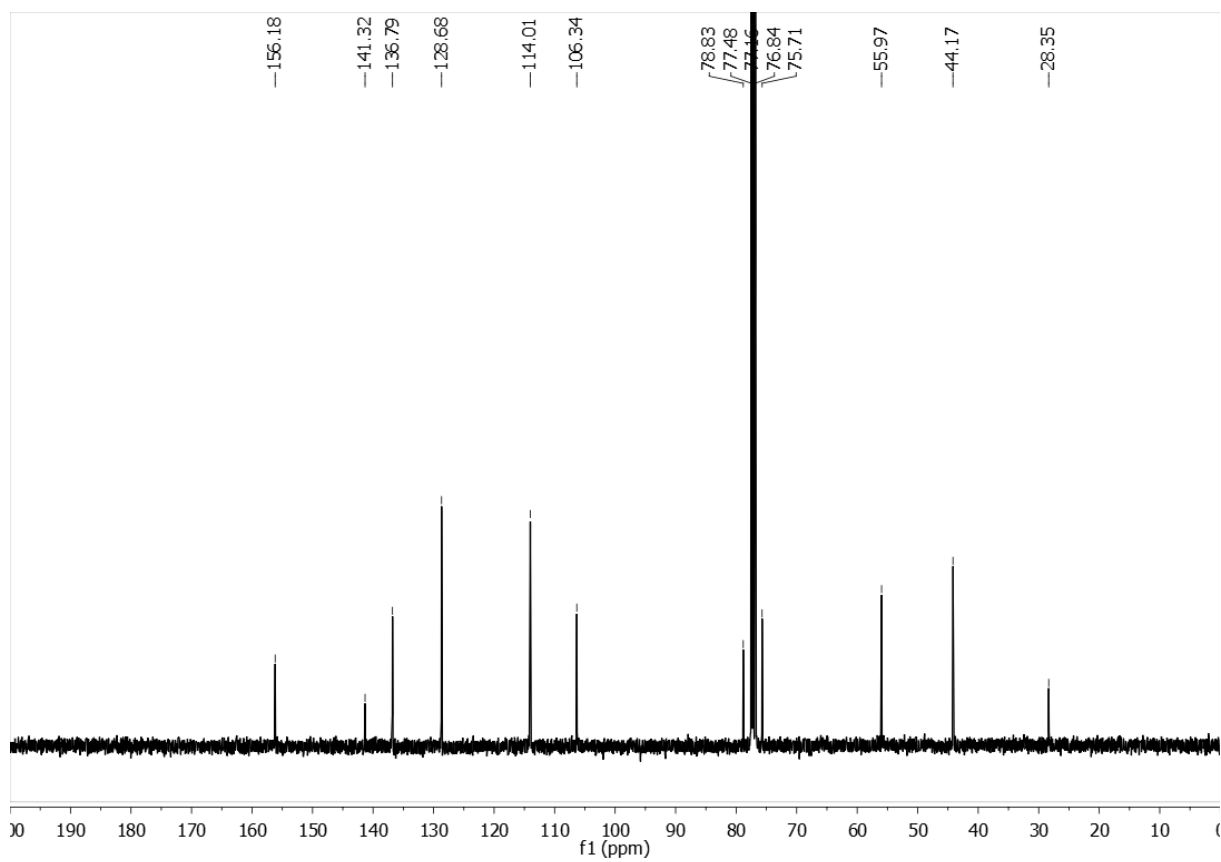
Figure 2: ^{13}\text{C} NMR spectrum (101 MHz, 298K) of CP2 in \text{CDCl}_3 .
