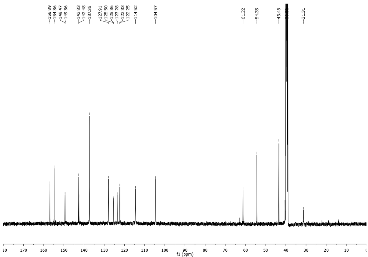
Figure 6: ^{13}\text{C} NMR spectrum (125 MHz, 298K) of CP3 in \text{d}_6\text{-DMSO} .
