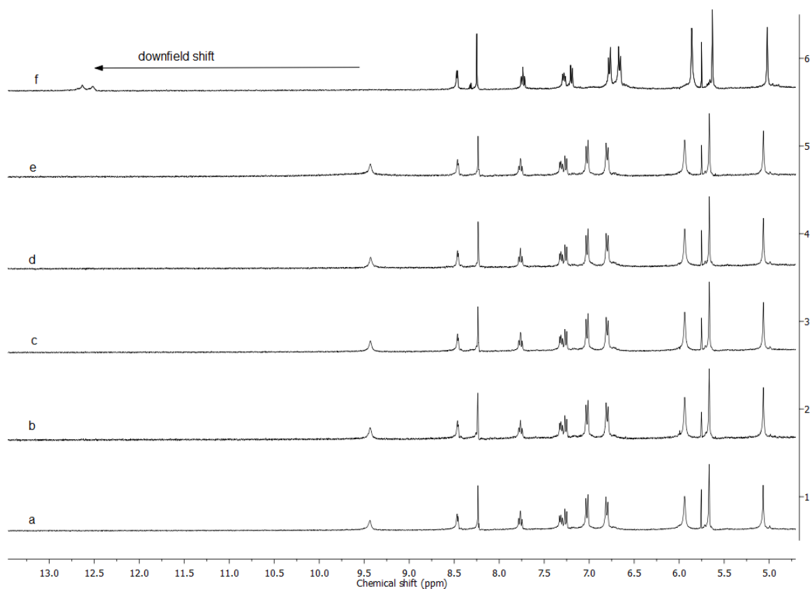
Figure 11 : ^1\text{H} NMR spectra for the titration of CP3 (a) in d_6 -DMSO with TBACl (b), TBABr (c), TBAI (d), TBAHSO 4 (e) and TBAF (f).
