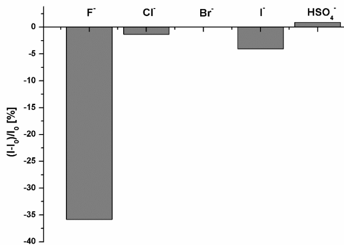
Figure 12 : Change in fluorescence emission of CP3 ( 5 \times 10^{-5} M, \lambda_{ex} = 300 nm, DMSO) upon addition of 10 equivalents of TBAF, TBACl, TBABr, TBAI and TBAHSO 4 .
