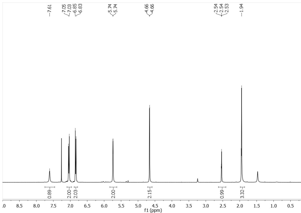
Figure 1: ^1\text{H} NMR spectrum (400MHz, 298K) of CP2 in \text{CDCl}_3 .
