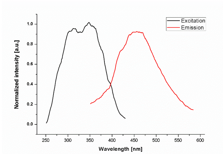
Figure 9 : Excitation and emission spectra of CP3 ( \lambda_{ex} = 300 nm, \lambda_{em} = 446 nm) in DMSO
