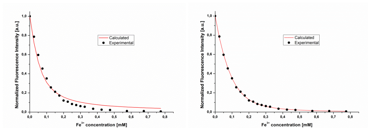
Figure 14: Fluorescence quenching of CP3 with \text{Fe}(\text{ClO}_4)_3 and calculated curve for A) 1:1 complex and B) mix of 1:1 and 1:2 complexes.
