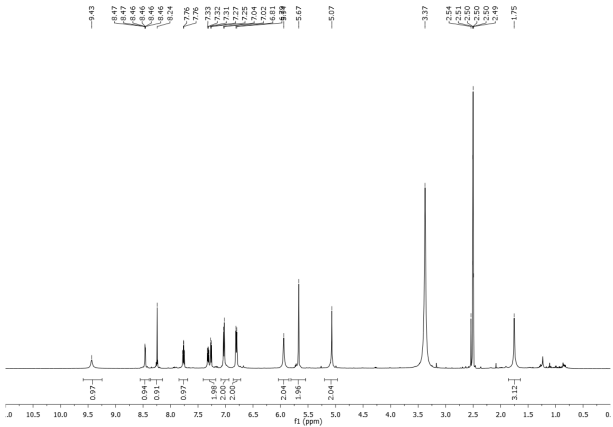
Figure 5: ^1\text{H} NMR spectrum (500MHz, 298K) of CP3 in \text{d}_6\text{-DMSO} .
