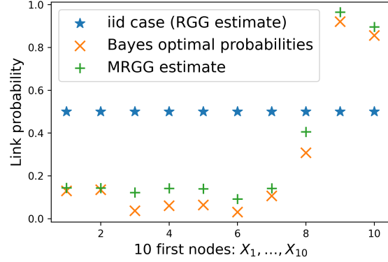
Figure 7. Link predictions between the future node X_{n+1} and the 10 first nodes X_1, \dots, X_{10} .
