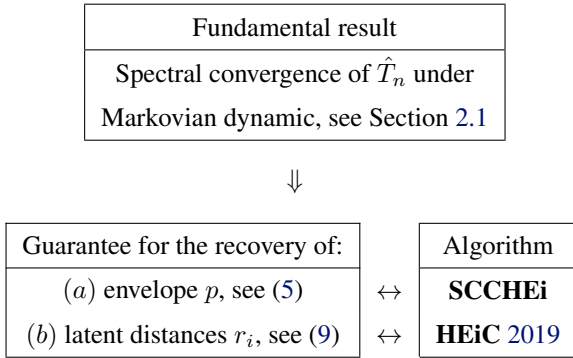
Figure 3. Presentation of our method to recover the envelope and the latitude functions.
