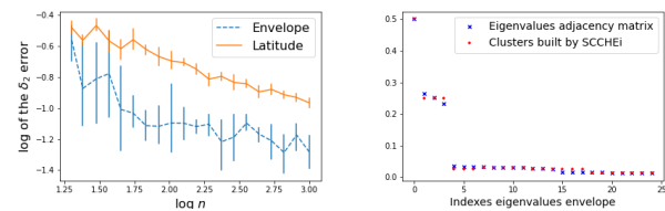
(a) \delta_2 error on envelope and lat-(b) Clustering adjacency eigenvalues ( R = 4 ).
