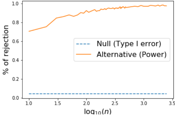
Figure 6. Hypothesis testing.
