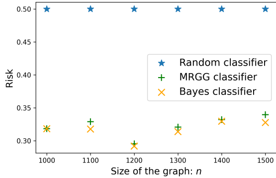
Figure 8. Comparison between the risk (defined in (13)) of the MRGG classifier, the random classifier and the risk of the optimal Bayes classifier.
