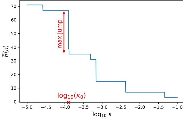
Figure 9. We sample the parameter \kappa on a logscale between 10^{-5} and 10^{-1} and we compute the corresponding R(\kappa) defined in (6). We plot the values of \tilde{R}(\kappa) with respect to \kappa . The larger jump allows us to define \kappa_0 .
