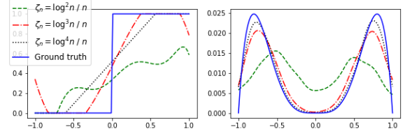
Figure 4. Results of our algorithms for graph of size 2,000 with functions of Eq.(10) and sparsity parameter \zeta_n = \log^k n/n , k \in \{2, 3, 4\} .
