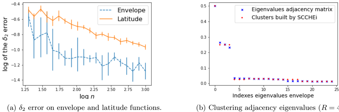
Figure 4: Non-parametric estimation of envelope and latitude using algorithms described in Sections 2 and 3. In (a), bars represent standard deviation of \delta_2 errors between true and estimated functions.
