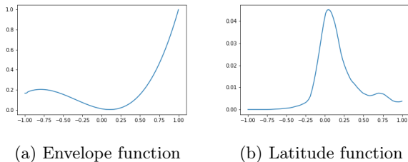
Figure 5: We run Algorithm SCCHEi with d = 3 and \hat{R} = 3 . Figure (a) shows the estimated function p which was rescaled in order to have 1 as maximum value on [0, 1] . For the latitude function, we removed 10% of the (\hat{r}_i)_i with the largest magnitude and we rescaled those remaining so that the maximum magnitude is 1. Normalizing to get a density on [-1, 1] , we obtain the latitude function presented in Figure 5 (b).
