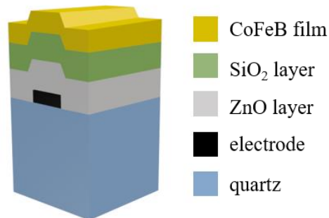
Fig. 10. The schematic of the CoFeB/SiO 2 /ZnO/quartz multi-layered structure.
