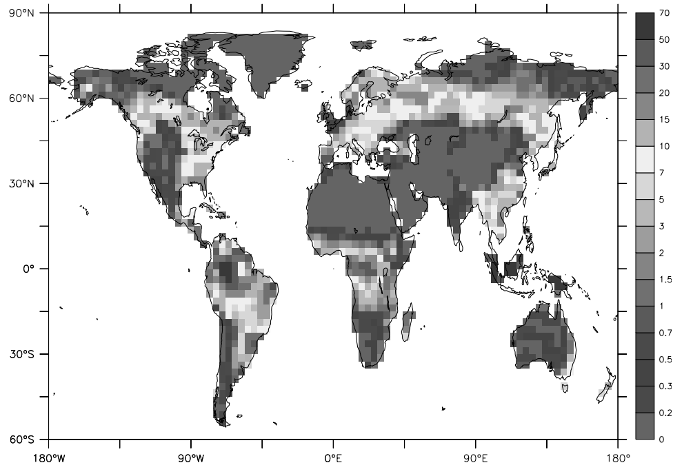
Figure 13. Mean aboveground and belowground biomass of natural vegetation (in \text{kgC}/\text{m}^2 ) in STAT. See color version of this figure at back of this issue.
