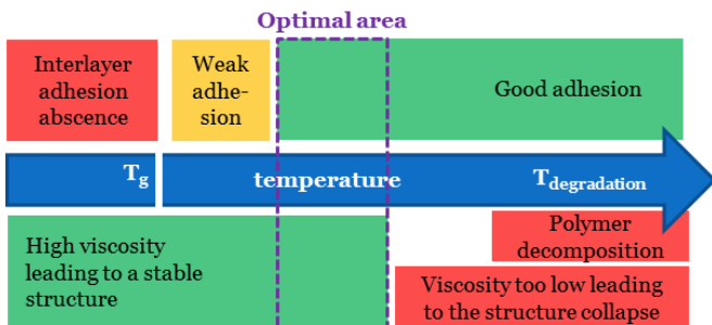
Fig. 1. Polymer printability rules for FFF process.
