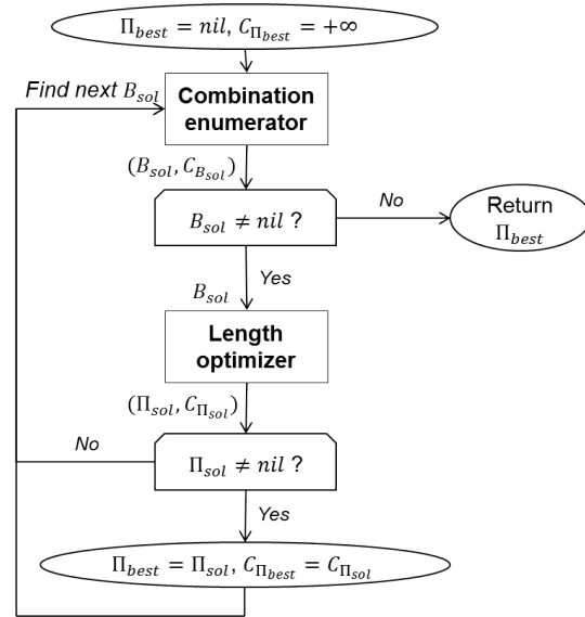
Figure 5: Architecture of the solver.
