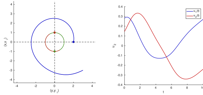
Fig. 2. Two vortices. Trajectory and control in the two vortices case. The initial adjoint vector being p_0 = (0.28, 0.15, 0.097, -0.47, -0.11, 0.088) (see Table 1 for details).
