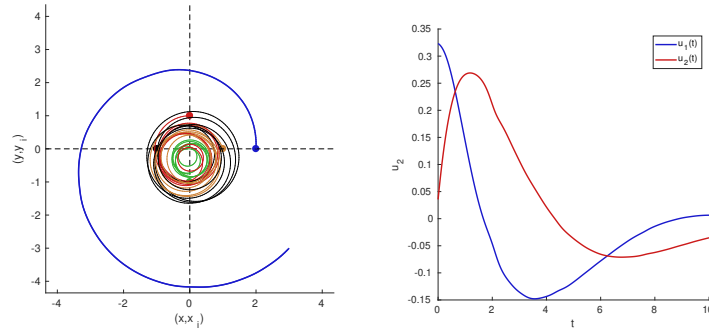
Fig. 4. Four vortices. Trajectory and control in the four vortices case. The initial adjoint vector is p_0 = (0.17, -0.0015, 0.041, -0.18, -0.025, -0.26, 0.11, 0.11, -0.18, 0.22) (see Table 1 for details).
