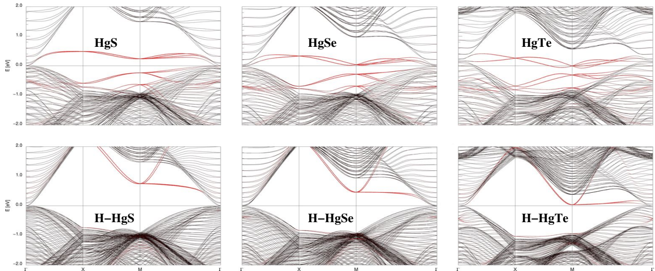
FIG. 3: (Color online) Band structures of (001) HgX-slabs with zincblende structure. Upper row: stacks of 8 cells with clean surfaces. Lower row: stacks of 12 cells with surfaces passivated by hydrogen. From the left to the right, results for \beta -HgS, HgSe, and HgTe are shown. The size of red dots on the bands indicates the band weight projected to the outermost HgX 2 (H-HgX 2 ) layers.
