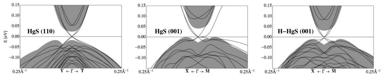
FIG. 2: Left: Band structure of a 9-cell (110) HgS-slab (lines) close to the \Gamma point along two specific directions, superimposed to the HgS bulk band structure (gray area) projected to the (110) surface; middle: the same for an 8-cell (001) HgS-slab (same data as published in Ref. 21); right: the same for an 12-cell H-passivated HgS-slab.
