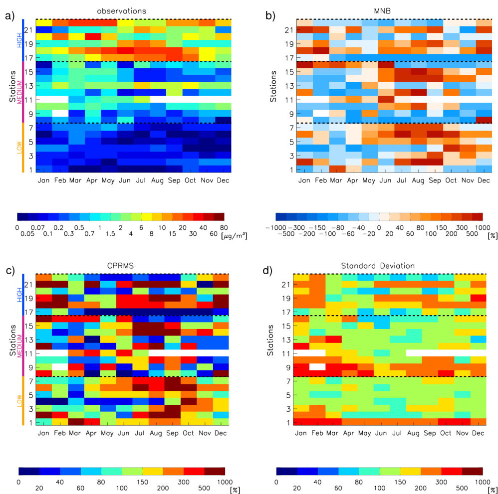
Fig. 6. Monthly averages of measured surface concentration in \mu\text{g m}^{-3} are shown together with the mean normalized bias (MNB), the normalized centred pattern root mean square error (CPRMS) and the normalized standard deviation (Sect. 2.4). In all subfigures, each row corresponds to the seasonal cycle at one of the stations and the row for each station corresponds to the number presented in Fig. 2. The stations have been grouped into Low (orange), Medium (violet) or High (blue) surface concentration sites (Sect. 2.2) and each group is identified by a colored bar on the left side of the left hand figures. Stations are ordered from south to north within each group. White color corresponds to months without measurements. For the individual figure of each model presenting the simulated values and their differences (in %) with respect to observations see Figs. S2 and S3, respectively, in the Supplement.
