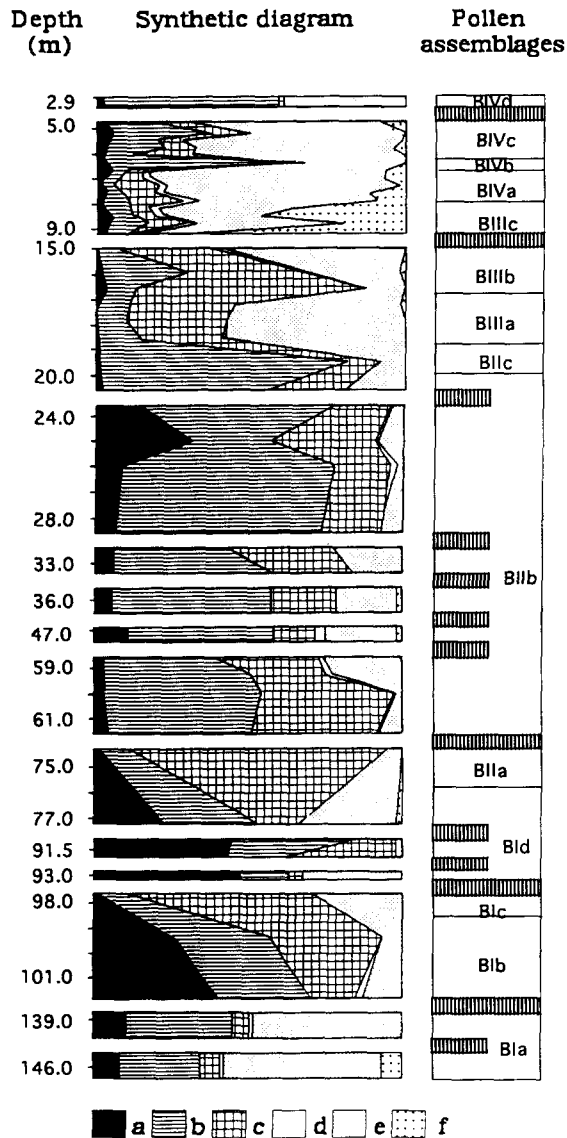
Fig. 2. Synthetic diagram of the Beune P&C core. a = Taxodiaceae, Taxodiaceae-Cupressaceae, Engelhardtia , Platycarya , Myrica , Myrtaceae; b = Carvy , Pterocarya , Quercus , Fagus , Carpinus , Ulmus , Alnus , Acer , Tsuga ...; c = Pinus , cf. Cathaya , cf. Cedrus ,... Abietaceae; d = Taxa without precise ecological significance (Rosaceae, Plantaginaceae, Labiatae,...); e = aquatic plants, Cyperaceae, Gramineae, Compositae, Amarantaceae-Chenopodiaceae, Caryophyllaceae, Ephedra ; f = Artemisia . (after Bachiri Taoufiq, 1988, modified) The dashed zones correspond to barren sediments.
