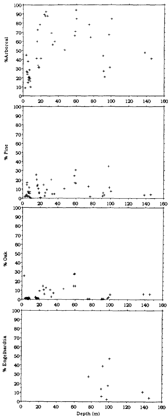
Fig. 4. Variations in total arboreal, Pinus , Quercus and Engelhardtia pollen percentages at the P & C Beaune core plotted against depth (in m).
