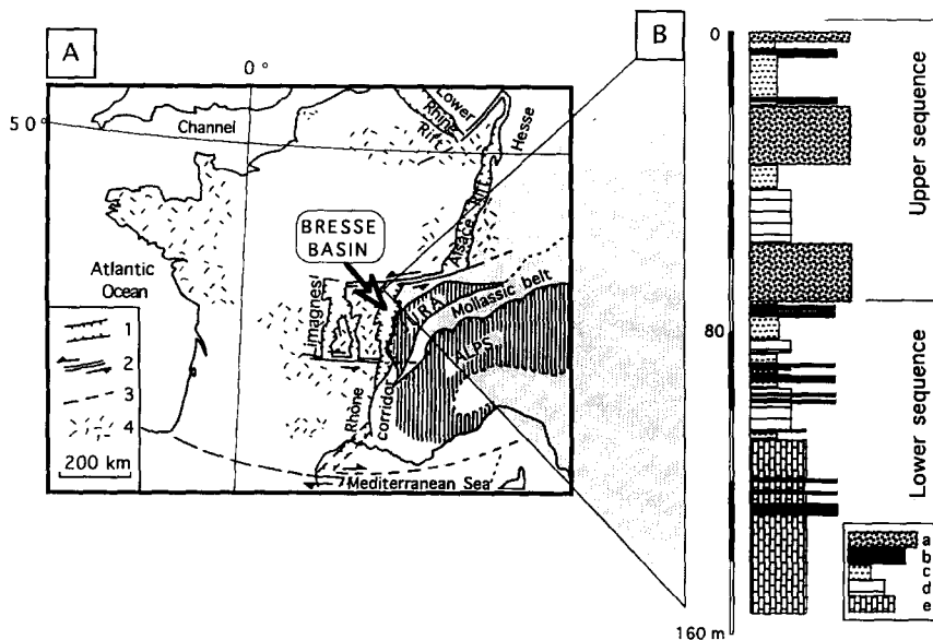
Fig. 1. A. Core location in Bresse Basin within the West-European rift. 1 = tectonic rift; 2 = transform zone; 3 = transform direction; 4 = outcrop areas of Hercynian substratum (after Rat, 1984, modified). B. Lithology of P & C core: a = calcareous; b = organic; c = shaly; d = silty; e = conglomeratic sediment (after Clair and Puisségur, 1988, modified).
