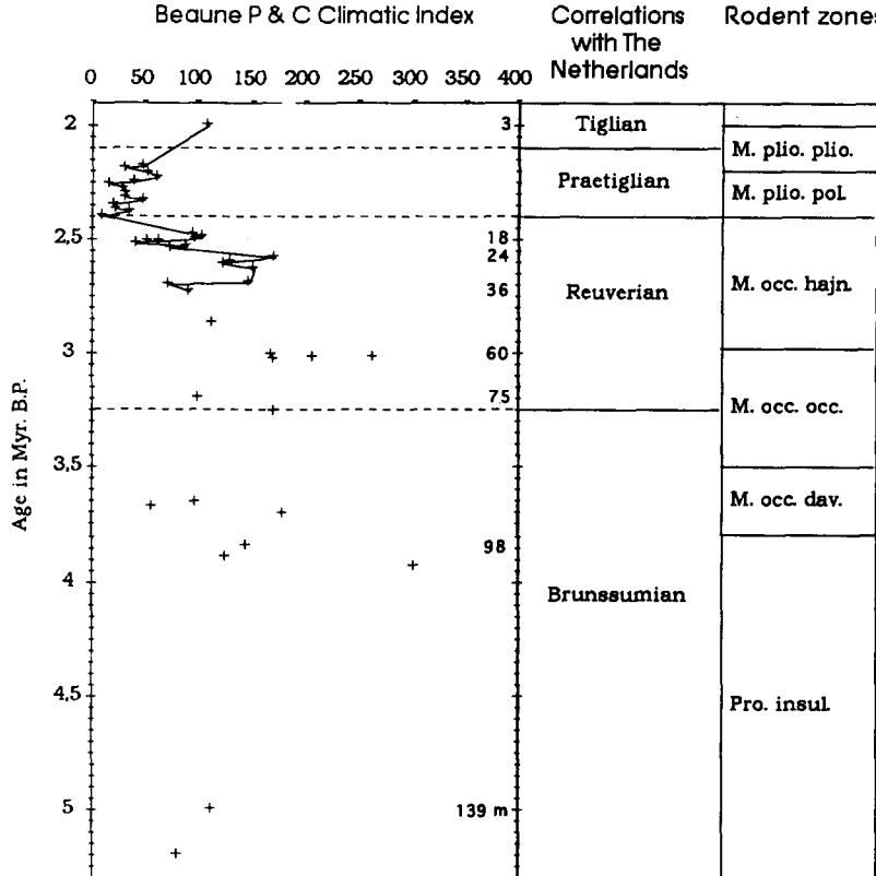
Fig. 5. Variations in Climatic derived Index (CI) at the P & C Core plotted against time and depth. Because of the poor preservation in the lower part of the core, the different calibrated levels were not joined up. The biostratigraphic scale is based on correlations between rodents and palynostratigraphy (after Chaline and Farjanel, 1990; Mein, 1990). M. plio. plio. = Mimomys pliocaenicus pliocaenicus ; M. plio. pol. = Mimomys pliocaenicus polonicus ; M. occ. hajn. = Mimomys occitanus hajnackensis ; M. occ. occ. = Mimomys occitanus occitanus ; M. occ. dav. = Mimomys occitanus davakosi ; Pro. insul. = Promimomys insuliferus .
