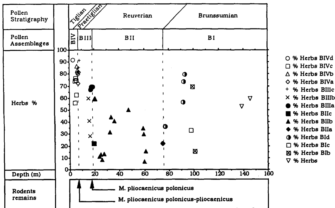
Fig. 3. Variations in herb pollen percentages against depth (in m) according to sporopollenic assemblages in European pollen stratigraphy. Location of rodent remains in the core. The different symbols correspond to the initial pollen groups determined by Bachiri Taoufiq (1988).
