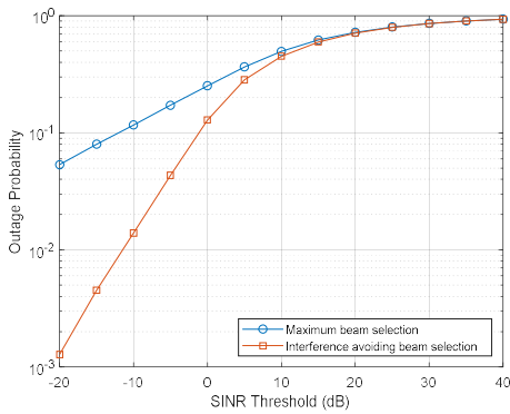
Figure 3. Outage probability vs. SINR threshold
