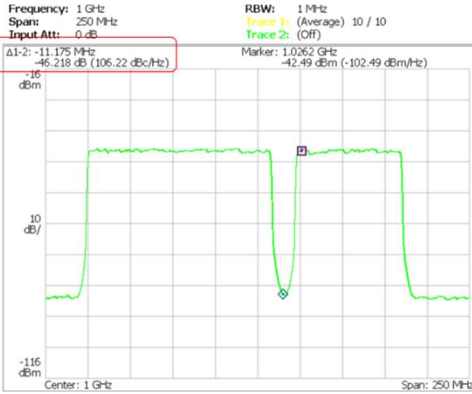
Figure 1. BF-OFDM spectrum
