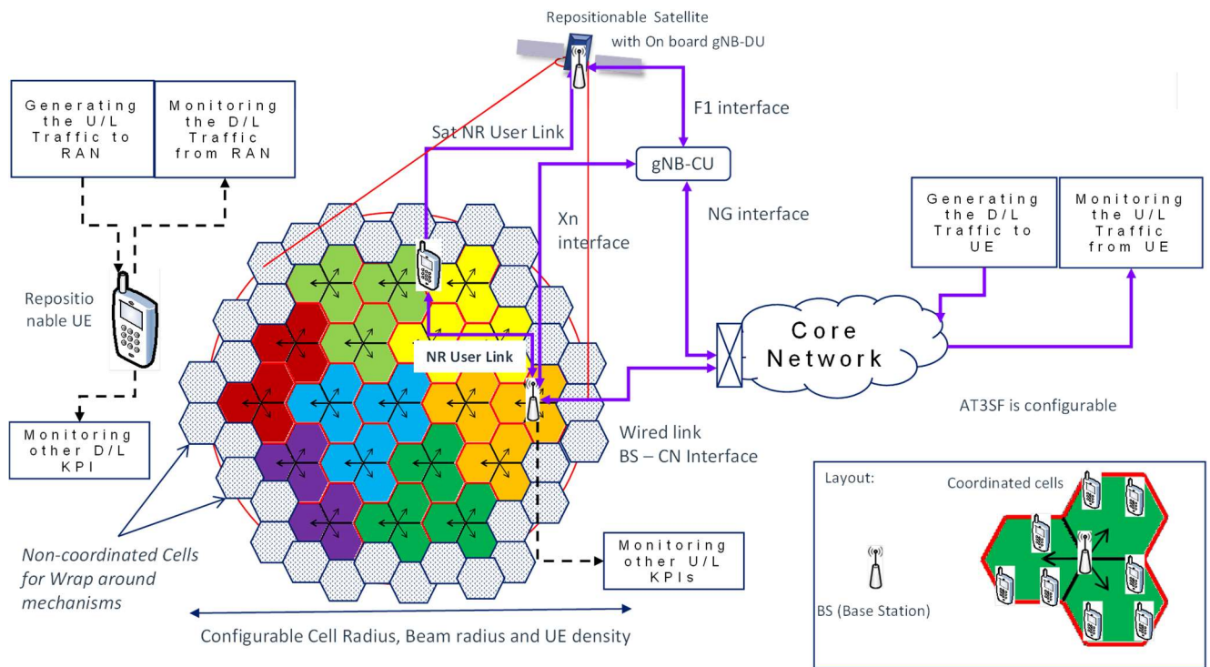
Figure 4. Architecture of the system as modeled in the RRM simulator. Overview.
