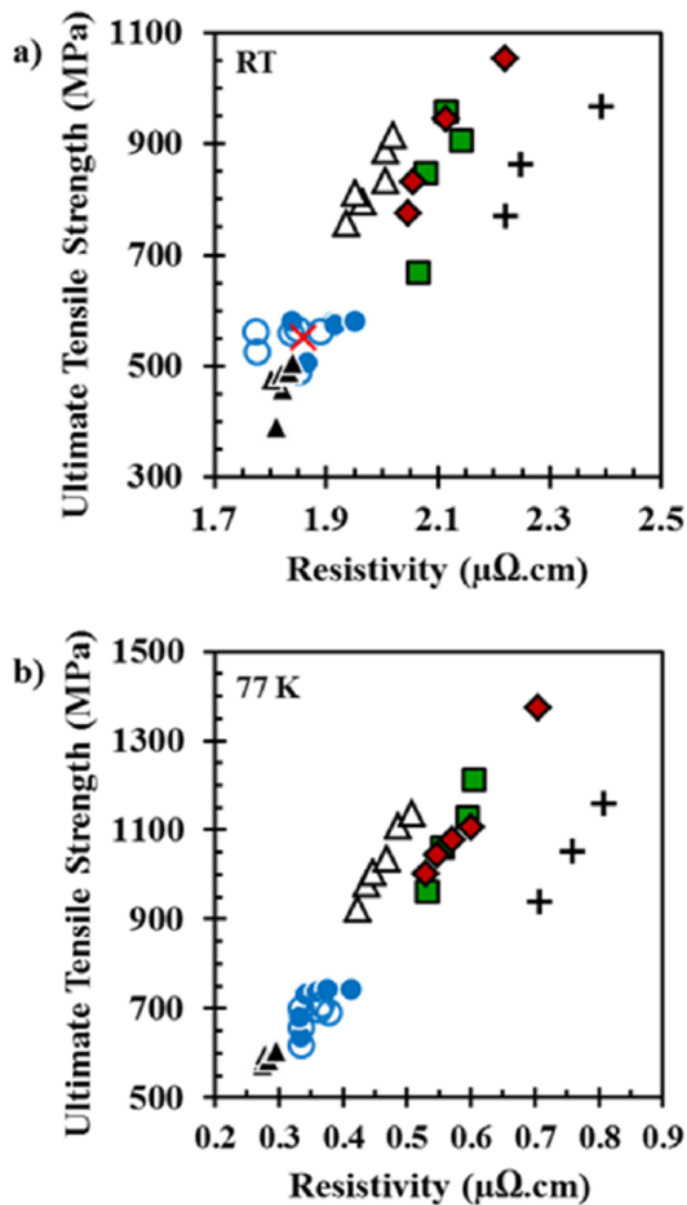
Fig. 4. Ultimate tensile strength versus electrical resistivity for a selection of the present Cu ( \blacktriangle ) and 1Ag-Cu/400 ( \triangle ), 5Ag-Cu/500 ( \blacksquare ), 10Ag-Cu/500 ( \blacklozenge ), CNT-Cu wires (1 % vol. CNT) [ \circ , \bullet ][5][6], Ag-Cu alloy wires (24 - 28 % wt. Ag) (+)[8]-[10], Ag-Cu cold spray alloy (5.7 % wt. Ag) ( \times )[13], (a) at 293 K and (b) at 77 K.
