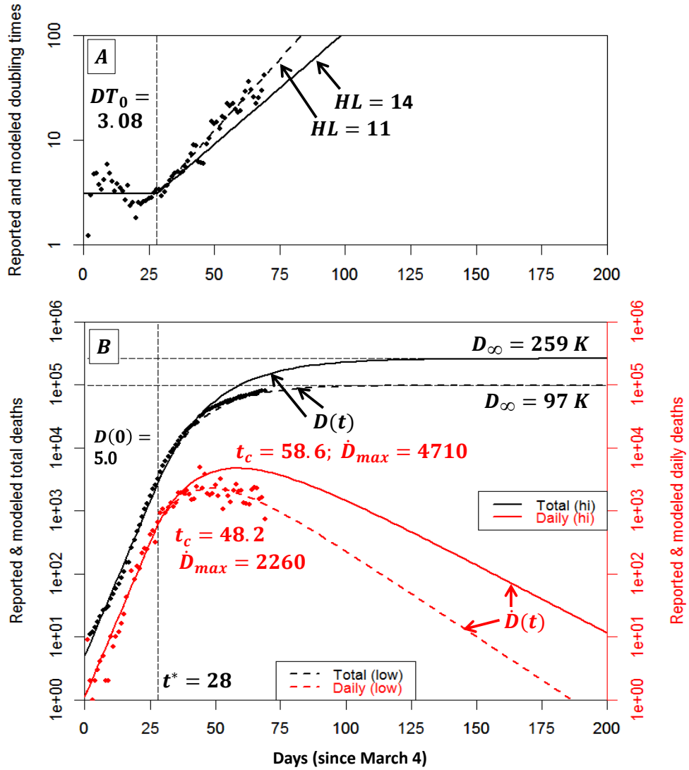
Figure 4: Panel A: Reported and low/high projected doubling times DT(t) for U.S. deaths from March 4 to May 11, 2020 (68 days). Panel B: Total reported and low/high projected total deaths D(t) in black; daily reported and low/high projected daily deaths \dot{D}(t) in red (semi-logarithmic scales).
