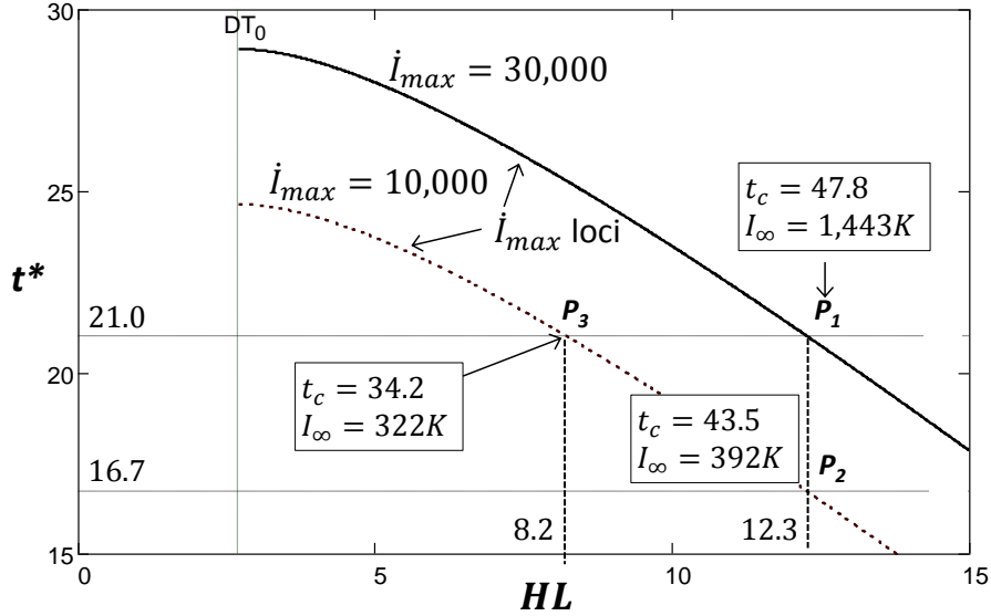
Figure 2: Loci of (HL, t^*) values for which the maximum incidence is \dot{I}_{max} = 10,000 and \dot{I}_{max} = 30,000 , with DT_0 = 2.3 , I(0) = 70 . A reduction from 30,000 to 10,000 is possible with (HL, t^*) moving from P_1 to P_2 with a 20% reduction of t^* . A move from P_1 to P_3 requires a 33% drop in HL but with more favorable outcomes concerning the timing t_c of the peak and the total number infected I_\infty .
