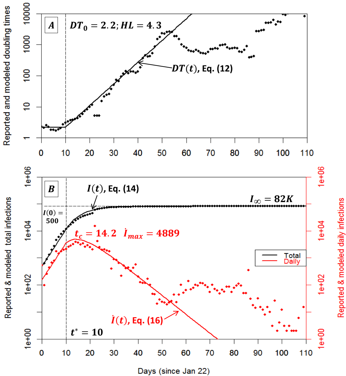
Figure 3: Panel A: Reported and modeled doubling times DT(t) in mainland China, from January 22 to May 11, 2020 (110 days). Panel B: Total reported and modeled numbers I(t) in black; daily reported and modeled numbers \dot{I}(t) in red (semi-logarithmic scales).
