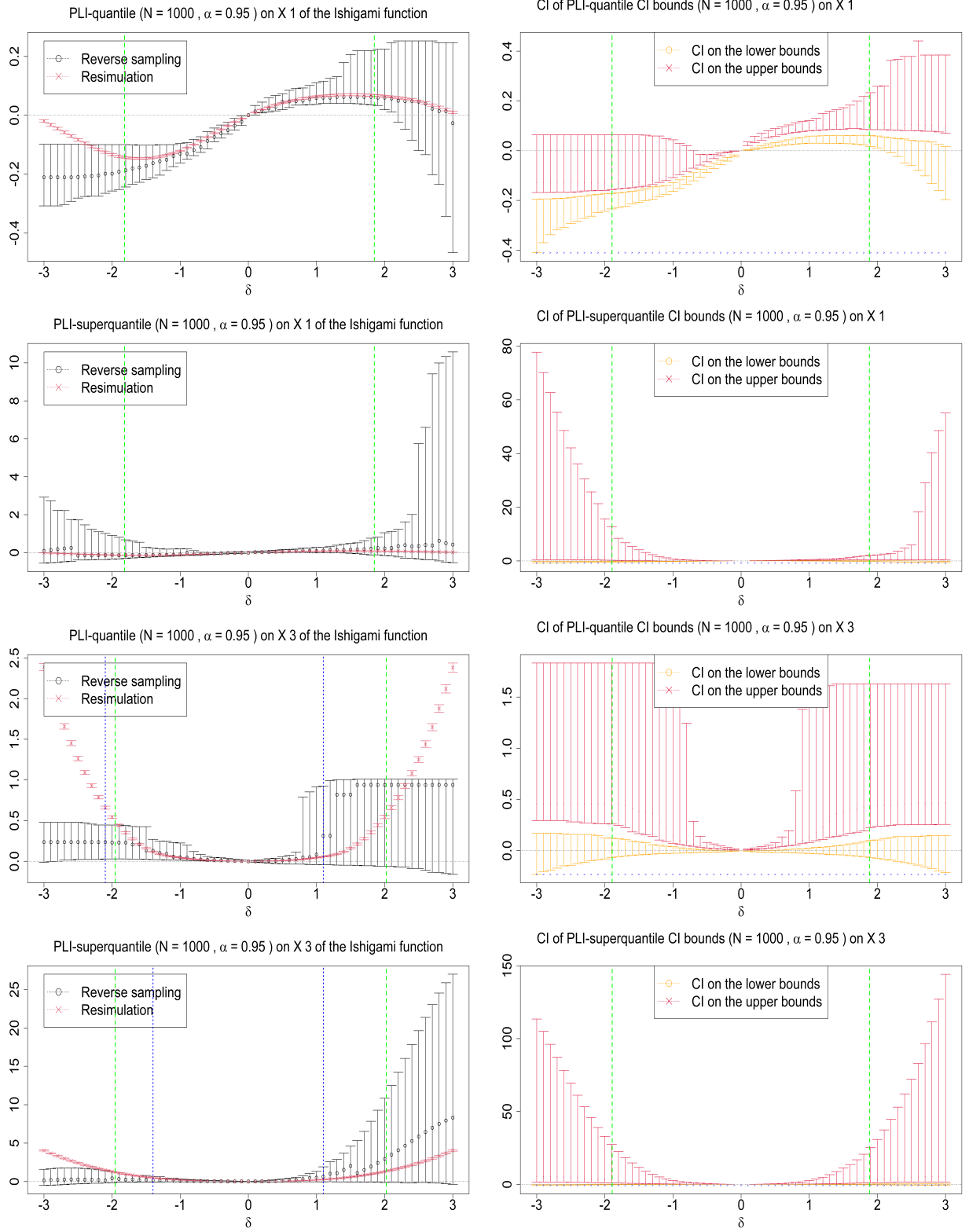
Figure 4: PLI validation results applied on X_1 and X_3 of the Ishigami function.
