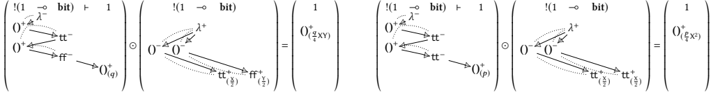
Fig. 9. Computing [[T]] \odot [[M_p, q]] \equiv O_{(\frac{q}{4}XY + \frac{p}{4}Y^2)}^+
