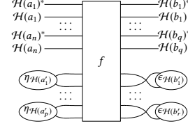
Fig. 7. Reduction \Downarrow_{x_A, x_B}(f)
