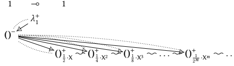
Fig. 8. The interpretation of \text{letrec } f^{1 \ominus 1} x^1 = X \cdot (\frac{1}{2} \cdot \text{skip} + \frac{1}{2} \cdot (f x)) in : 1 \ominus 1
