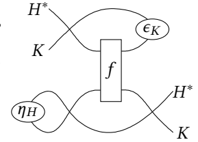
Fig. 3. Construction of \bar{f}
