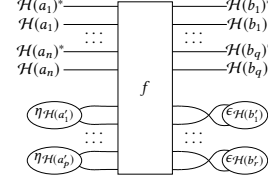
Fig. 7. Reduction \Upsilon_{x_A, x_B}(f)
