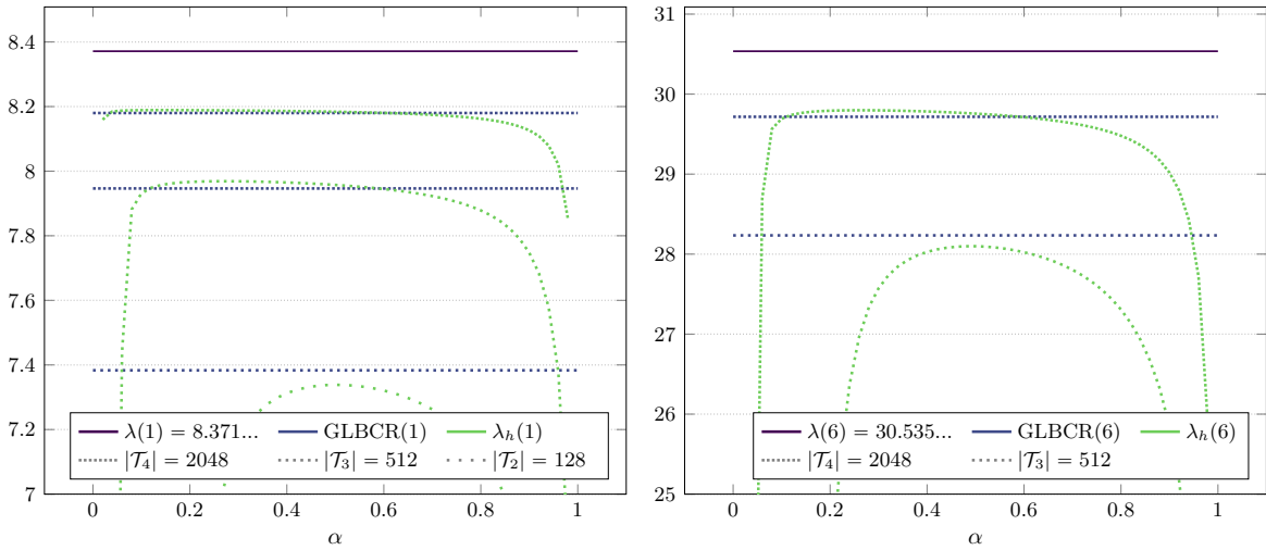
Figure 7.5: Slit domain: comparison of \text{GLBCR}(j) and \lambda_h(j) for parameter \alpha varying in (0, 1) and \beta = (\alpha - \delta^2 \lambda_{\text{CR}}(j)) / \sigma^2 \in (0.001, 0.198) on coarse uniform triangulations.
