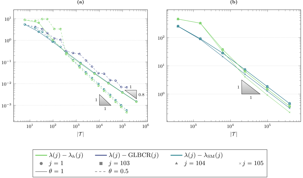
Figure 7.2: L-shaped domain: comparison of the distance between \lambda(j) and \lambda_h(j) (computed with \alpha = 0.4, \beta = 0.07 (left) and \beta = 0.06 (right)), \text{GLBCR}(j) [CG14b], and \lambda_{\text{SM}}(j) [CZZ20] computed on uniform ( \theta = 1 , solid) and adaptive ( \theta = 0.5 , dashed) meshes with (7.2). Left: \lambda(1) . Right: \lambda(103) = \lambda(104) = \lambda(105) .
