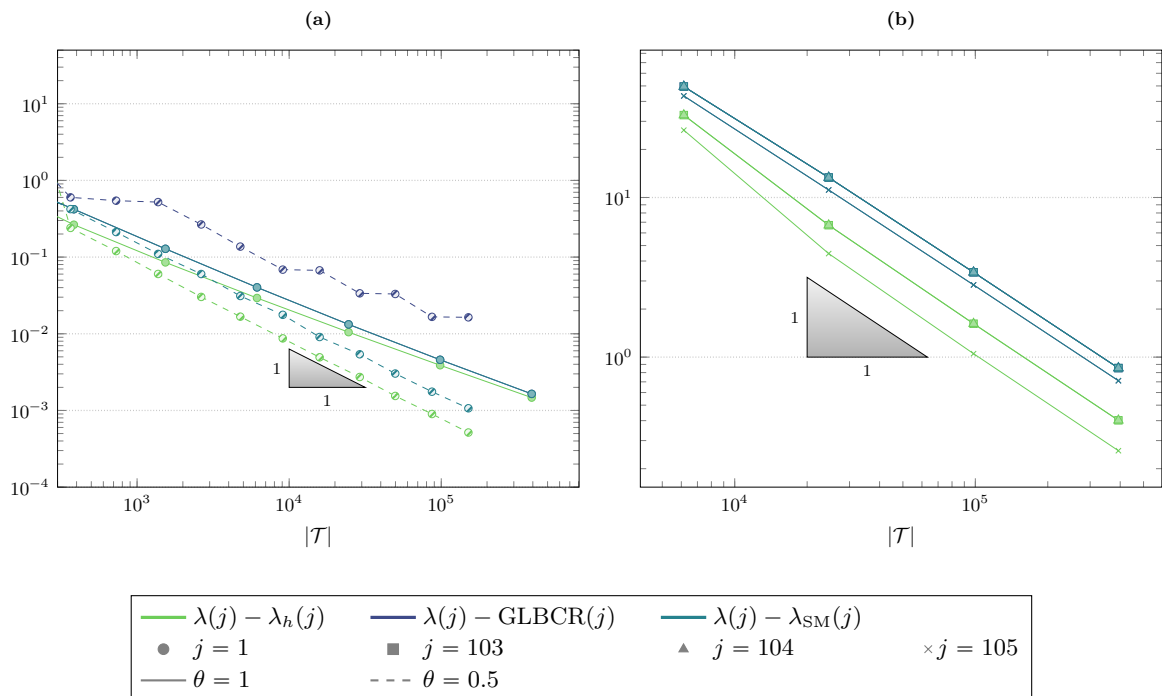
Figure 7.2: L-shaped domain: comparison of the distance between \lambda(j) and \lambda_h(j) (computed with \alpha = 0.5 , \beta = 0.08 ), \text{GLBCR}(j) [CG14b], and \lambda_{\text{SM}}(j) [CZZ19] computed on uniform ( \theta = 1 , solid) and adaptive ( \theta = 0.5 , dashed) meshes with (7.2). Left: \lambda(1) . Right: \lambda(103) = \lambda(104) = \lambda(105) .
