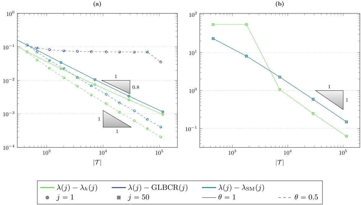
Figure 7.6: First isospectral domain: comparison of the distance between \lambda(j) and \lambda_h(j) (computed with \alpha = 0.5 , \beta = 0.08 ), \text{GLBCR}(j) , and \lambda_{\text{SM}}(j) . Left: \lambda(1) . Right: \lambda(50) .
