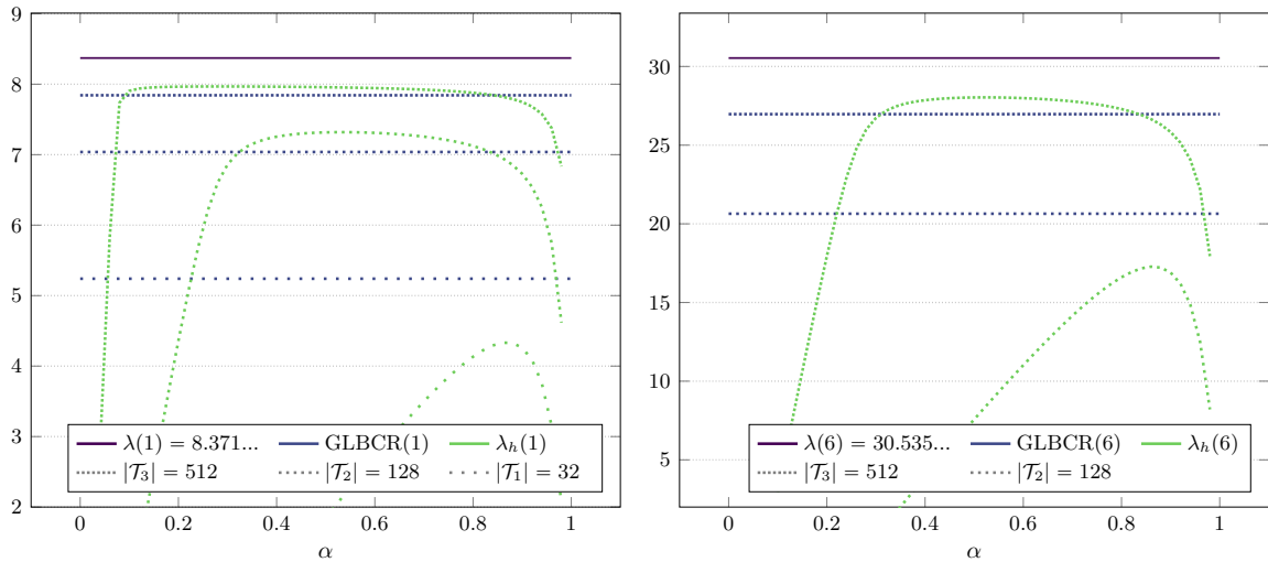
Figure 7.5: Slit domain: comparison of \text{GLBCR}(j) and \lambda_h(j) for parameter \alpha varying in (0, 1) and \beta = (\alpha - \delta^2 \lambda_{\text{CR}}(j))/\sigma^2 \in (0.003, 0.196) on coarse uniform triangulations.
