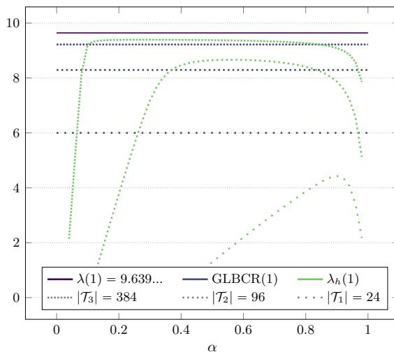
Figure 7.3: L-shaped domain: comparison of GLBCR(1) and \lambda_h(1) for parameter \alpha varying in (0, 1) and \beta = (\alpha - \delta^2 \lambda_{\text{CR}}(1))/\sigma^2 \in (0.003, 0.195) on coarse uniform triangulations.
