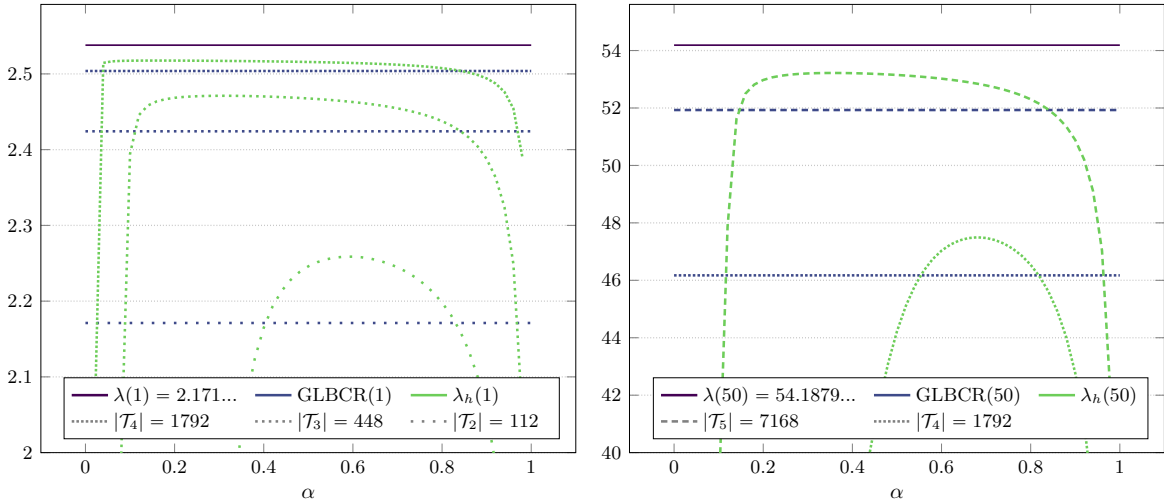
Figure 7.7: First isospectral domain: comparison of \text{GLBCR}(j) and \lambda_h(j) for parameter \alpha varying in (0, 1) and \beta = (\alpha - \delta^2 \lambda_{\text{CR}}(j))/\sigma^2 \in (0.0026, 0.198) .
