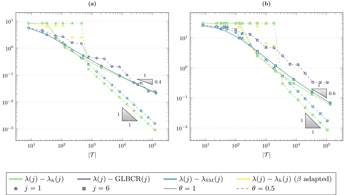
Figure 7.4: Slit domain: comparison of the distance between \lambda(j) and \lambda_h(j) (computed with \alpha = 0.5 , \beta = 0.08 ), \text{GLBCR}(j) [CG14b], and \lambda_{\text{SM}}(j) [CZZ19] computed on uniform ( \theta = 1 , solid) and adaptive ( \theta = 0.5 , dashed) meshes with (7.2). Left: \lambda(1) . Right: \lambda(6) .
