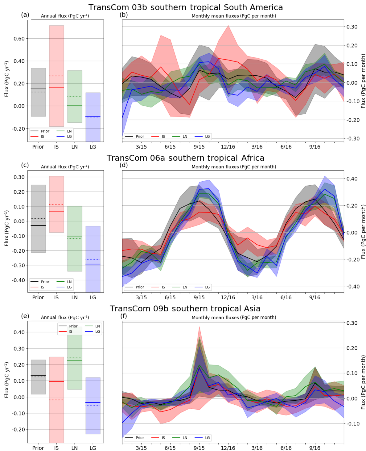
Figure 7. As in Fig. 3, but for selected terrestrial regions in the southern tropics on different continents. Among the three continents, satellite-derived posterior fluxes differ substantially from the prior and in situ constrained fluxes only in tropical Africa, where the peak outgassing is shifted later in the year by a few months.
