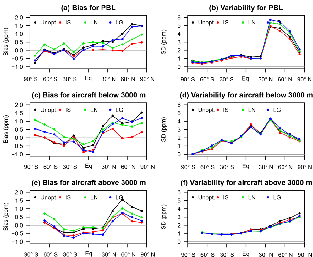
Figure 9. Comparisons between in situ measurements and unoptimized and optimized posterior concentrations using different observational constraints. Panels (a), (c), and (e) depict the overall bias and (b), (d), and (f) the standard deviation of the errors, each plotted against latitude. The rows distinguish between measurements in the PBL (a, b), aircraft below 3000 m a.s.l. (c, d), and aircraft above 3000 m (e, f). Aircraft measurements include the NOAA light aircraft profiles (Sweeney et al., 2015), CONTRAIL flask and analyzer data, and observations from the ORCAS and Atom campaigns. The PBL measurements were assimilated in the IS experiments, which is apparent given the very low bias in (a, b) for the red curve. The IS experiments exhibit the smallest bias throughout the atmosphere in the northern extratropics and above the PBL in the southern extratropics (largely driven by ORCAS data), while the LN posterior concentrations have the lowest bias above the PBL in the tropics. LG posterior concentrations in general follow the unoptimized concentrations, with a slight negative or positive shift that depends on latitude and altitude. None of the observational constraints improves the match to the variability in the observations much over the prior mean.
