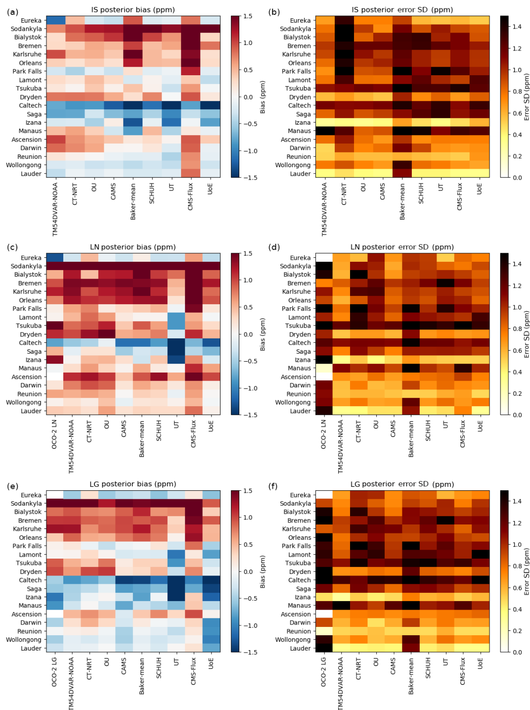
Figure 8. Bias (a, c, e) and standard deviation (b, d, f) for all TCCON sites by model (ordered by latitude). Statistics are computed from all residuals: simulated – retrieved X_{CO_2} . For the OCO-2 LN (c, d) and OCO-2 LG (e, f) statistics, the first column depicts the statistics for the residuals between collocated OCO-2 10 s values and TCCON retrievals. Of note is the correlation between the bias in the OCO-2 retrievals and the resultant bias in the posterior concentrations. In general, LN experiment posterior samples show a high bias relative to TCCON at all except a few sites. IS and LG show similar biases over most of the sites. According to O’Dell et al. (2018), land nadir observations are biased high by about 0.5 ppm relative to land glint observations. The LN experiment also has a larger standard deviation at most TCCON sites than the IS and LG experiments. Of particular interest are the various European sites, for which all models and data constraints show a high bias relative to TCCON.
