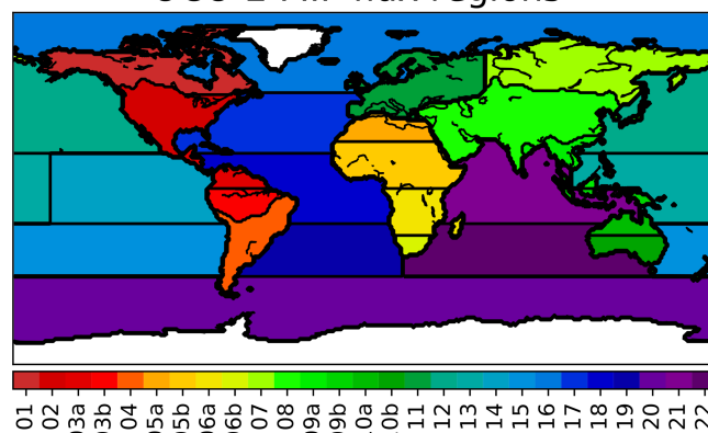
Figure 2. Regions on which prior and posterior gridded fluxes are aggregated for comparison.
