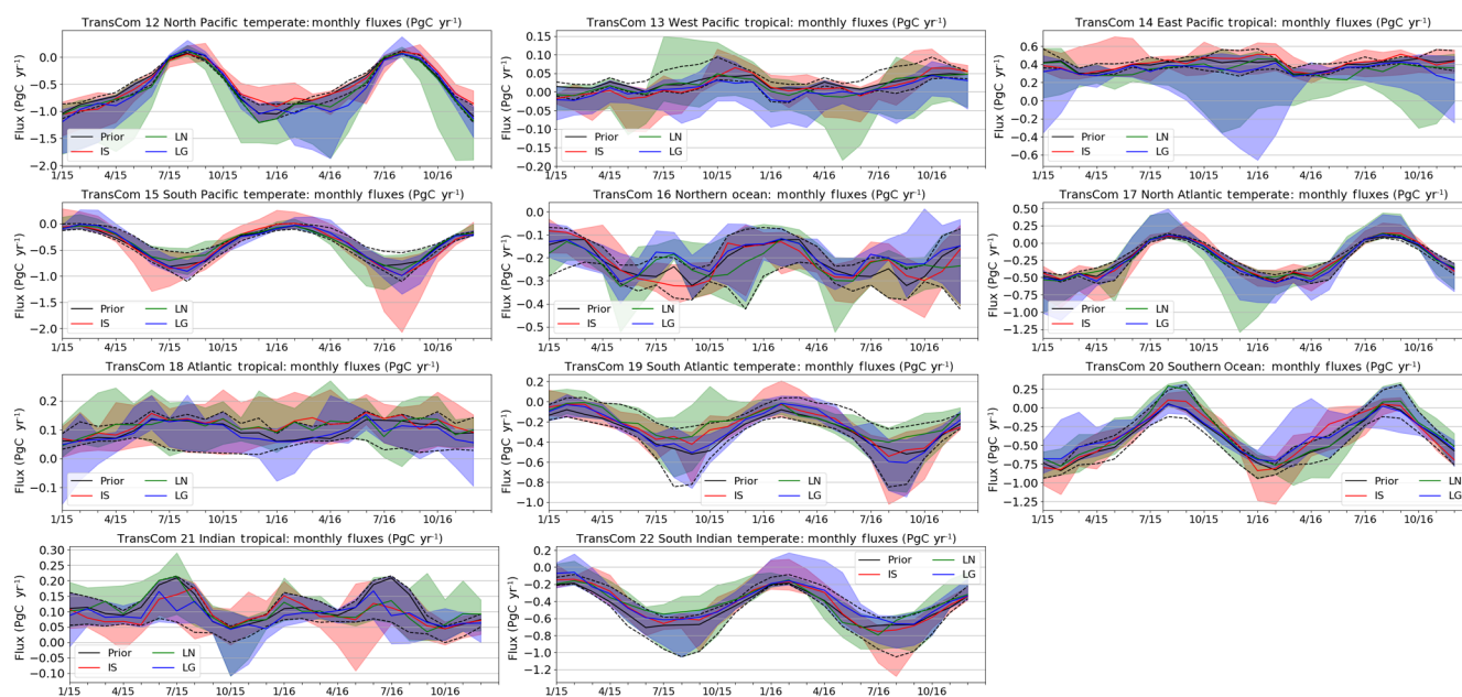
Figure B4. As in Fig. B3, but for the 11 Transcom ocean regions.
