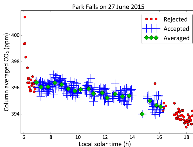
Figure C1. An example of TCCON X_{\text{CO}_2} retrievals at Park Falls on 27 June 2015. Red circles denote retrievals that were rejected by the outlier filter, SZA filter, and TCCON flagging, while blue plus signs denote retrievals that passed those filters. Green diamonds denote the 30 min averages of the accepted retrievals that were eventually used by the modelers for this study.
