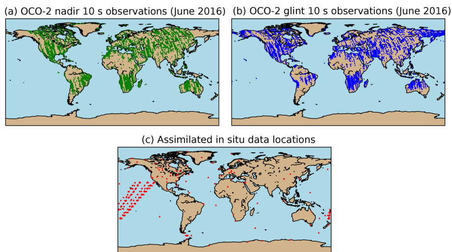
Figure 1. Sample locations of different data sources described in the text: locations of OCO-2 nadir (a) and glint (b) 10 s retrievals for June 2016; in situ assimilation data (c).
