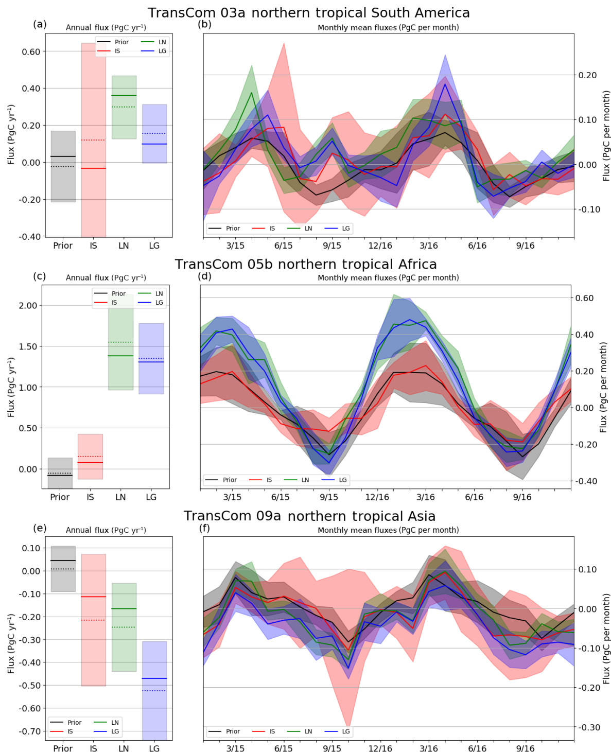
Figure 6. As in Fig. 3, but for selected terrestrial regions in the northern tropics on different continents. Among the three continents, satellite-derived posterior fluxes differ substantially from the prior and in situ-constrained fluxes only in northern tropical Africa, where the outgassing in the dry season is about double the magnitude. The phasing in the posterior fluxes is also different in southern tropical Africa, where the peak outgassing is shifted later in the year by a few months.
