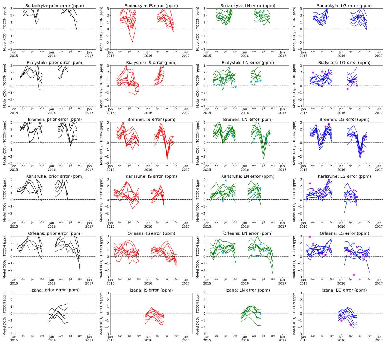
Figure C3. As in Fig. C2, but for European TCCON sites.
