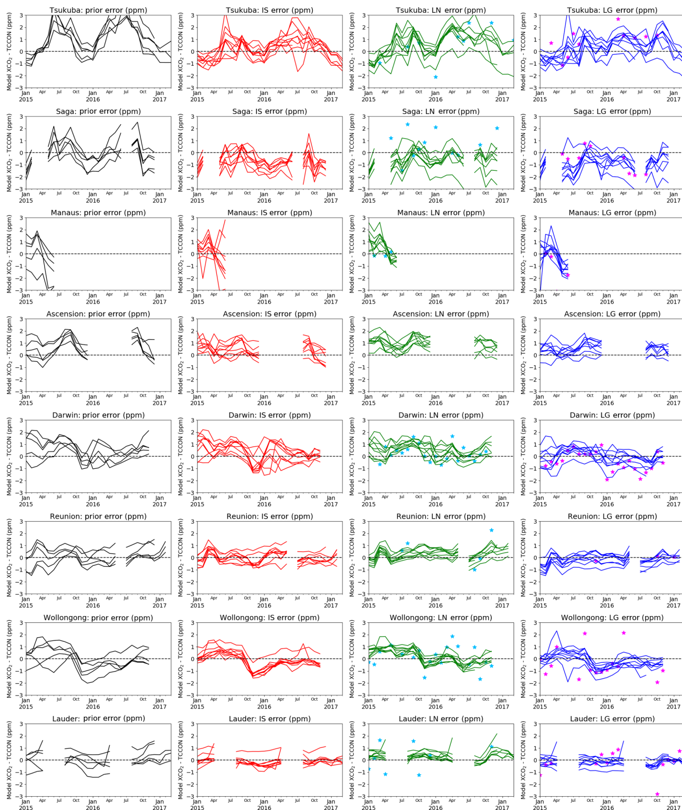
Figure C4. As in Fig. C2, but for sites in Japan, the tropics, and the Southern Hemisphere.
