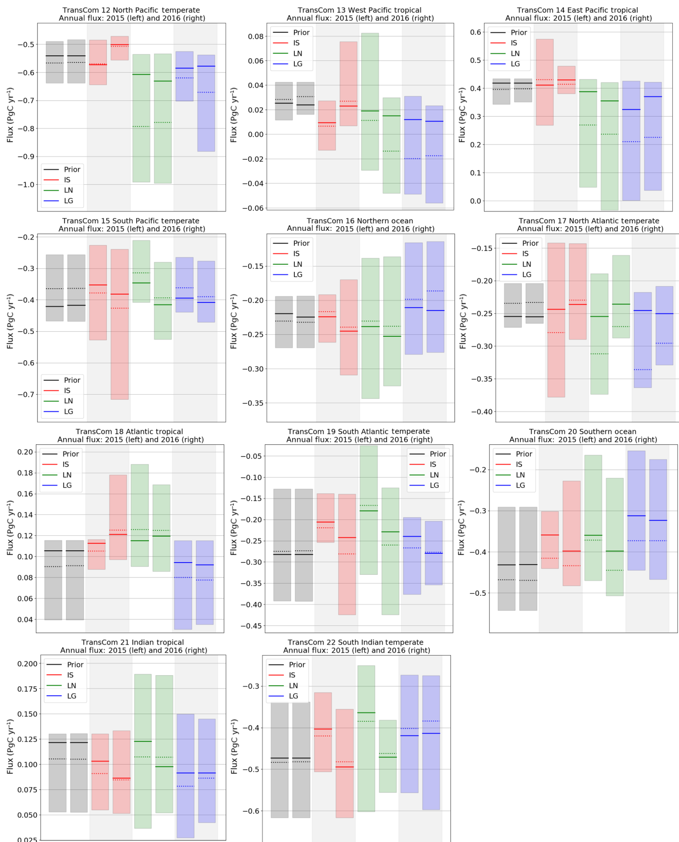
Figure B2. As in Fig. B1, but for the 11 Transcom ocean regions.
