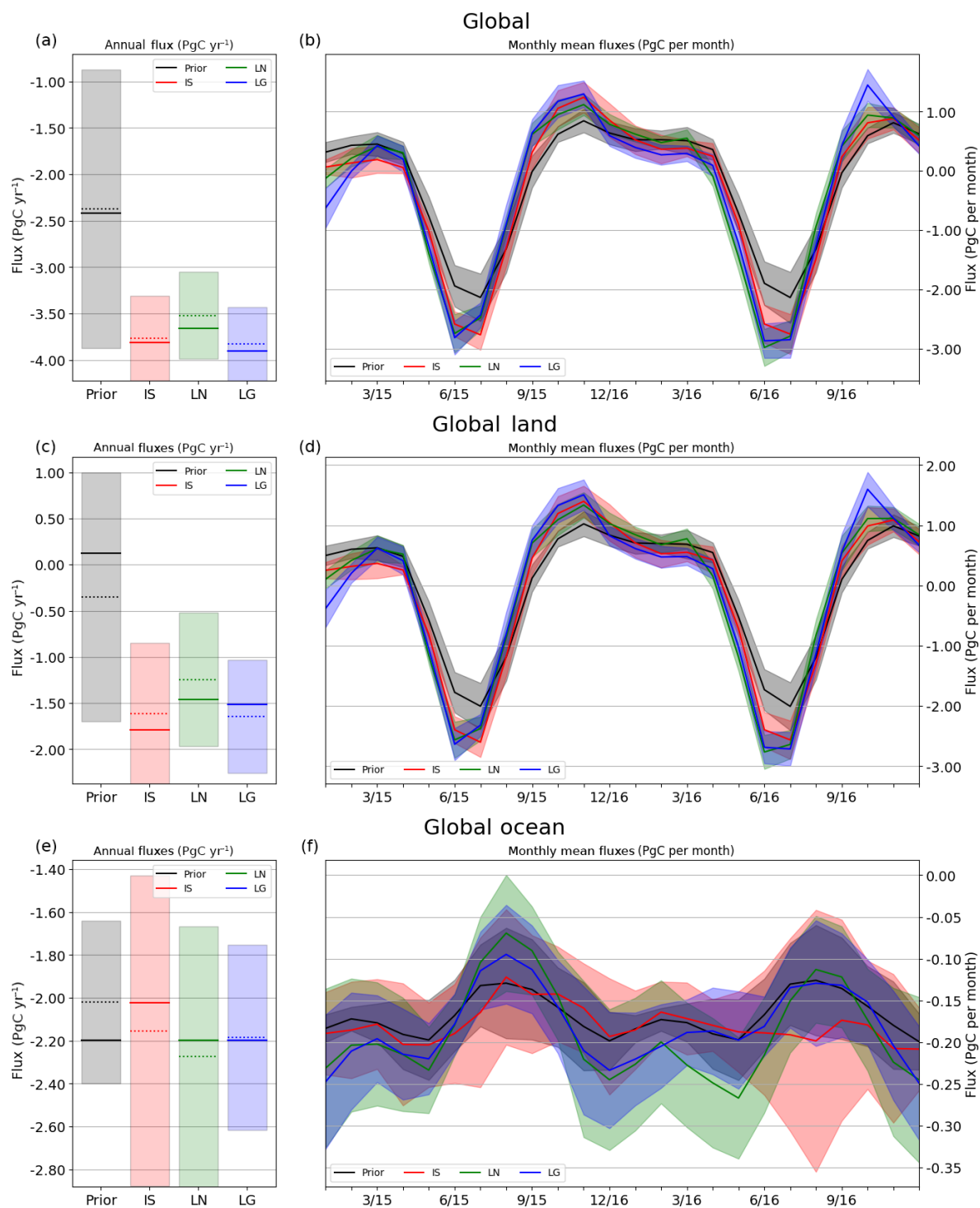
Figure 3. Prior (black) and posterior 2015–2016 mean (a, c, e) and monthly (b, d, f) fluxes constrained by in situ (red), OCO-2 land nadir (green), and OCO-2 land glint (blue) observations. (a, c, e) The shaded bar represents 1 standard deviation of the model ensemble about the ensemble mean annual mean flux (dashed line). The solid horizontal line for each bar depicts the median of the ensemble annual mean fluxes. (b, d, f) For each time series, the solid line represents the mean of the OCO-2 MIP ensemble, while the shading represents the ensemble standard deviation.
