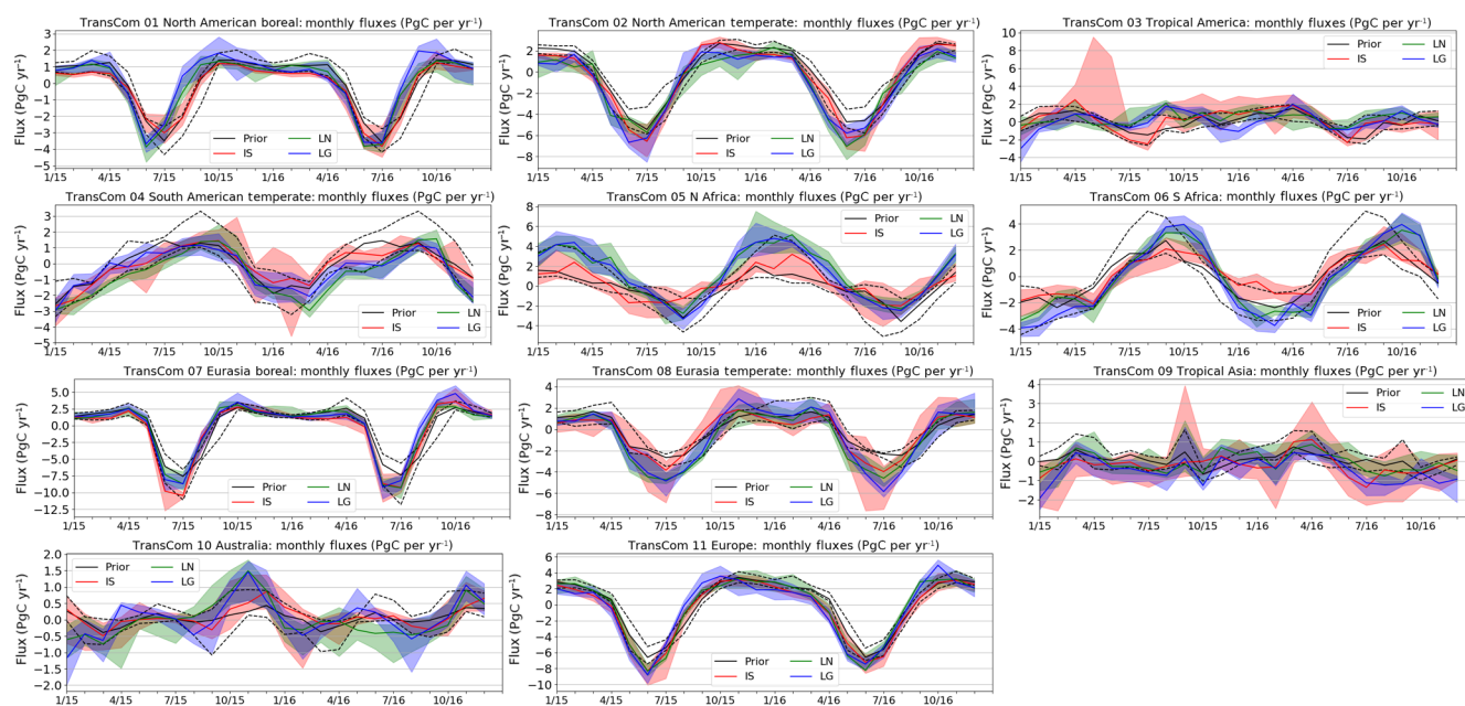
Figure B3. As in Fig. B1, except that the fluxes are by month.
