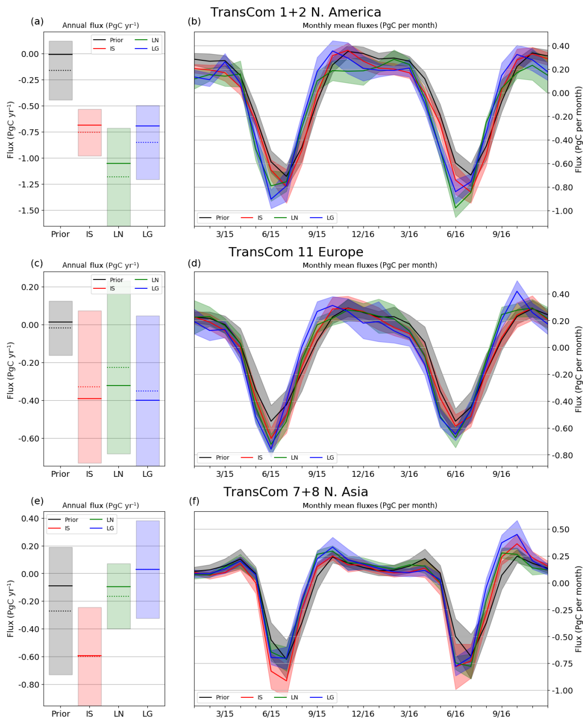
Figure 5. As in Fig. 3, but for three continental-scale land regions in the northern extratropics. The monthly fluxes show broad agreement between the in situ and OCO-2 experiments in terms of seasonality and peak drawdown. The fluxes show differences in North America, where the summertime peak sink is larger and wintertime respiration is smaller in the LN experiment results than the other two. The three experiments agree for Europe, which diverges from results in Houweling et al. (2015) in which GOSAT retrievals lead to a much stronger sink in Europe than the in situ measurements. In both Europe and Asia, LG experiment results display the enhanced outgassing in the autumn in 2016 present in the northern extratropics seen in Fig. 4.
