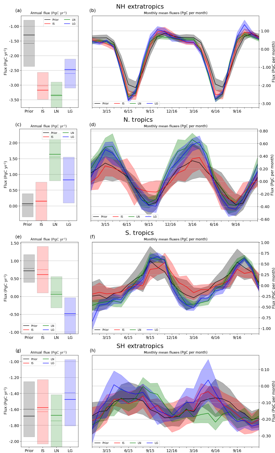
Figure 4. As in Fig. 3, but for zonal regions described by intervals of latitude: 23–90° N (Northern Hemisphere extratropics), 0–23° N (northern tropics), 23° S–0° (southern tropics), 90–23° S (southern hemisphere extratropics). As in the case of global land, posterior net fluxes in the northern extratropics all demonstrate a larger peak drawdown as well as a different seasonality from the prior, with the net drawdown period beginning earlier and ending earlier. The satellite retrievals imply a much more dynamic seasonality than either the prior or the in situ-constrained fluxes, particularly in the tropics, where the amplitudes of the seasonal cycles are significantly larger.
