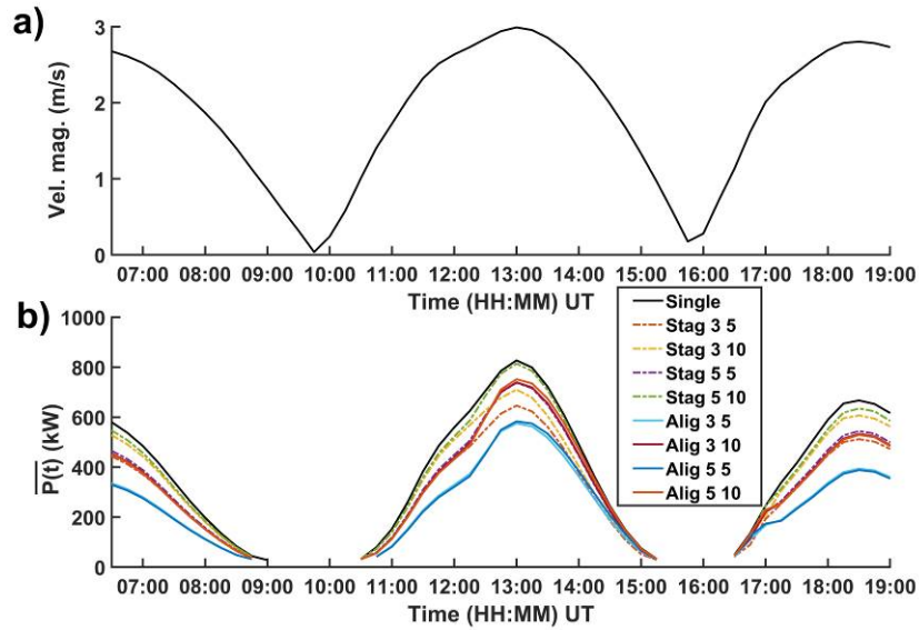
Figure 6: a) Temporal evolution of the velocity magnitude during the selected period. b) Temporal evolution of the output per turbine (total output divided by the number of turbines).
