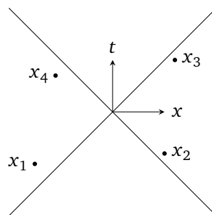
Figure 5.5: Regge kinematics.
