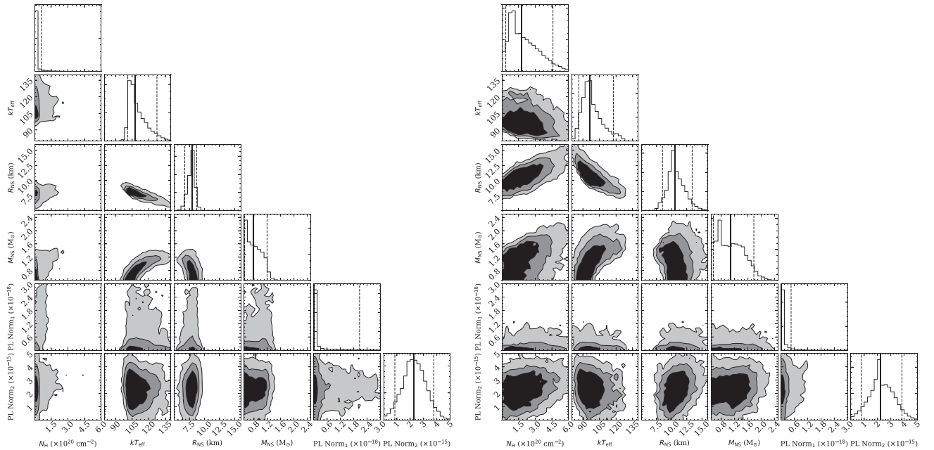
Figure 4. The one- and two-dimensional MCMC posterior distributions for the parameters in the spectral fitting (Section 3.2). The black, dark grey, and light grey regions correspond to the 68 per cent, 90 per cent, and 99 per cent credible intervals, respectively, for the nsatmos H-atmosphere (left) and nsx He-atmosphere (right) models. The solid line in the one-dimensional posterior distributions represents the median value, while the left/right dashed lines represent the 5 per cent and 95 per cent percentiles, respectively. Note that in the mass parameter the lower limit is technically unconstrained, since it is consistent with the hard limit of nsatmos and nsx models. In both figures, the power-law normalization of group 1 (PL Norm 1 ) and group 2 (PL Norm 2 ) are measured in units of \text{erg s}^{-1} \text{cm}^{-2} .
