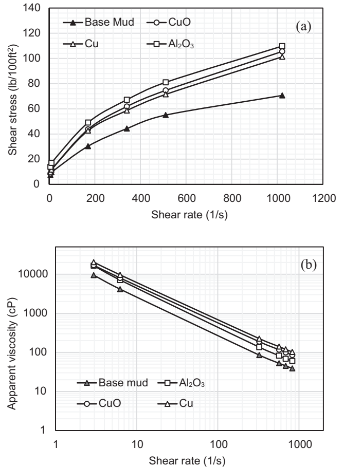
Fig. 6. (a) Shear stress and (b) the apparent viscosity versus shear rate for various drilling nanofluids.
