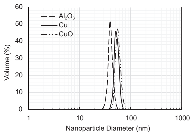
Fig. 3. Particle size distribution of nanoparticles.
