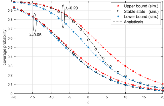
Figure 2. Comparison of Monte Carlo simulation and analytically iterative algorithm of coverage probability at stable state.
