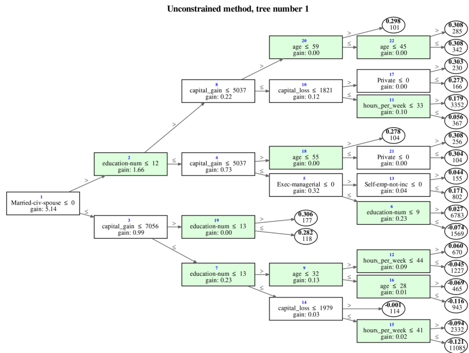
unconstrained method
