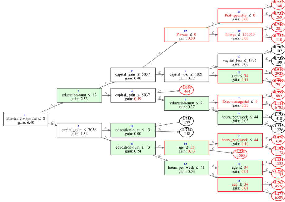
Constrained LightGBM tree, tree number 1
