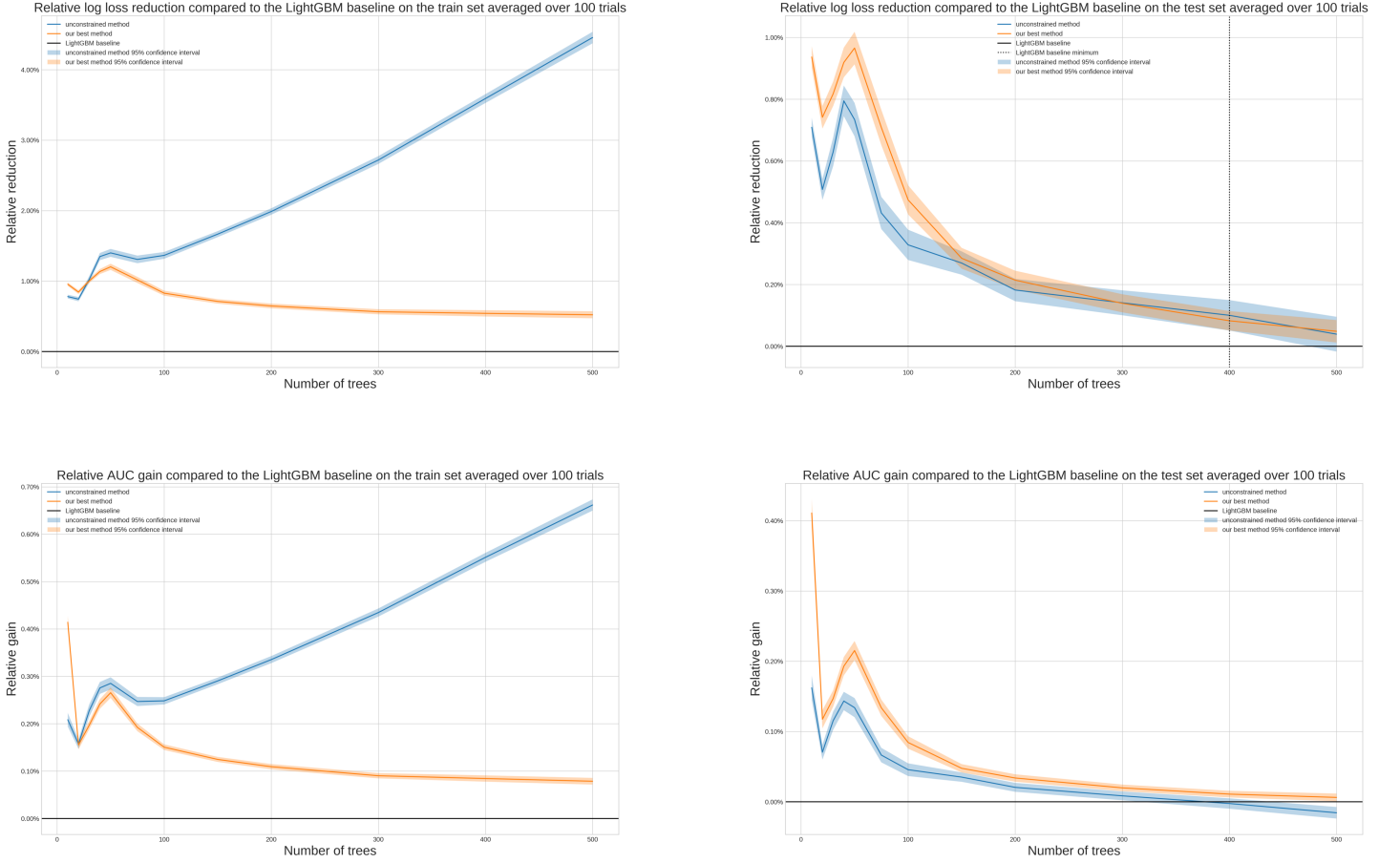
Figure 1: Loss and AUC vs. number of iterations relative to the constrained LightGBM baseline, for our best method and the unconstrained method, on the train and test sets
