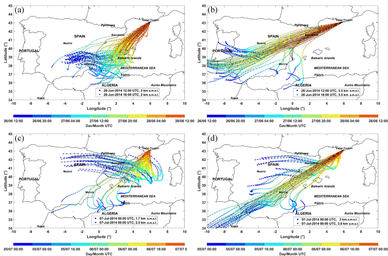
Figure 10. 2-day back trajectories from the French Riviera (Toulon; 43.13556° N, 6.00944° E). The altitudes of the end locations of the air mass trajectories are in the main pollution plumes detected by the ground-based N 2 -Raman lidar on (a) 28 June 2014 for an end location of 2 km, (b) 28 June 2014 for an end location of 3.5 km, (c) 7 July 2014 for end locations of 1.7 and 2.5 km, and (d) 7 July 2014 for end locations of 3 and 3.8 km. The HYSPLIT model worked in its ensemble mode, i.e., 27 back trajectories computed for each end location.
