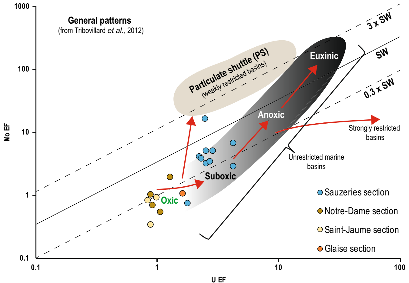
FIGURE 11 Plot of U-EF versus Mo-EF for the GL samples showing the oxygenation conditions in the Goguel Level. The SW line corresponds to the Mo/U molar ratios similar to the seawater value (SW ~7.5 to 7.9) and the dashed lines correspond to the fractions thereof ( 3 \times \text{SW} , 0.3 \times \text{SW} ). The pattern of U and Mo EFs are compared to the model proposed in Algeo and Tribovillard (2009)
