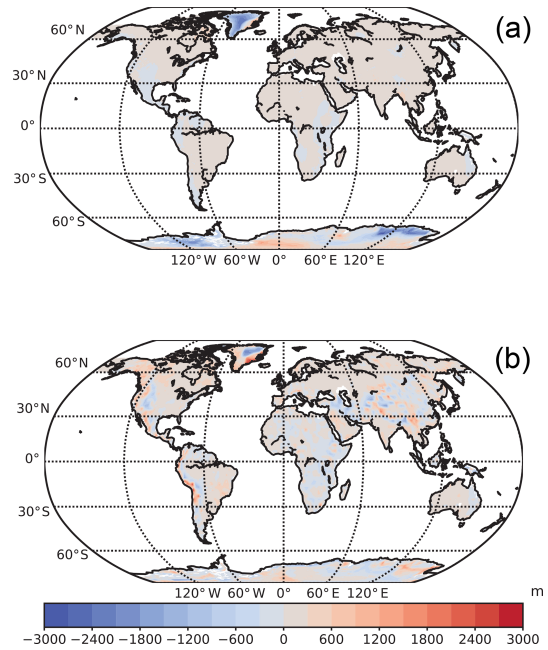
Figure 1. Anomalies of the Pliocene topography relative to PI control (a) and Pliocene 1 (b).
