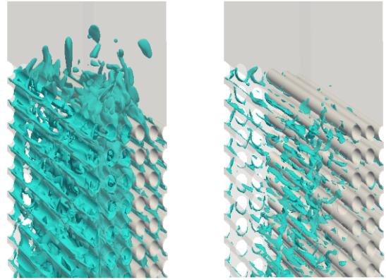
FIGURE 8: Instantaneous void fraction contours of 30% (left) and 36% (right), DISP approach.
