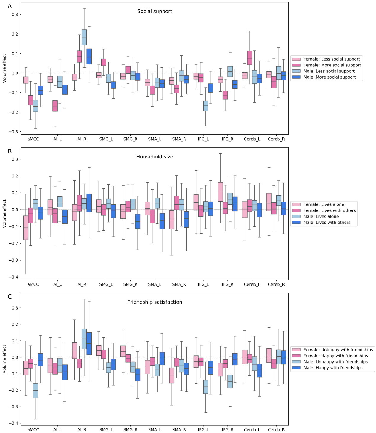
Figure 4. Population volume effects in the intermediate-level network of the social brain. Boxplots depict four different subgroups in the context of (A) social support, (B) number of people living in the same household and (C) friendship satisfaction. (A) Volume effects were incongruent in the anterior midcingulate cortex (aMCC), left anterior insula (AI_L), left supramarginal gyrus (SMG_L), right supplementary motor area (SMA_R), right inferior frontal gyrus (IFG_R) and left cerebellum (Cereb_L) in women with more social support and in the anterior midcingulate cortex (aMCC), right anterior insula (AI_R) and left inferior frontal gyrus (IFG_L) in men with less social support. (B) Men living with others displayed volume effects in the right supramarginal gyrus (SMG_R) and left supplementary motor area (SMA_L) compared to men living alone. (C) Men who are not happy with their friendships showed large volume effects in the anterior midcingulate cortex
