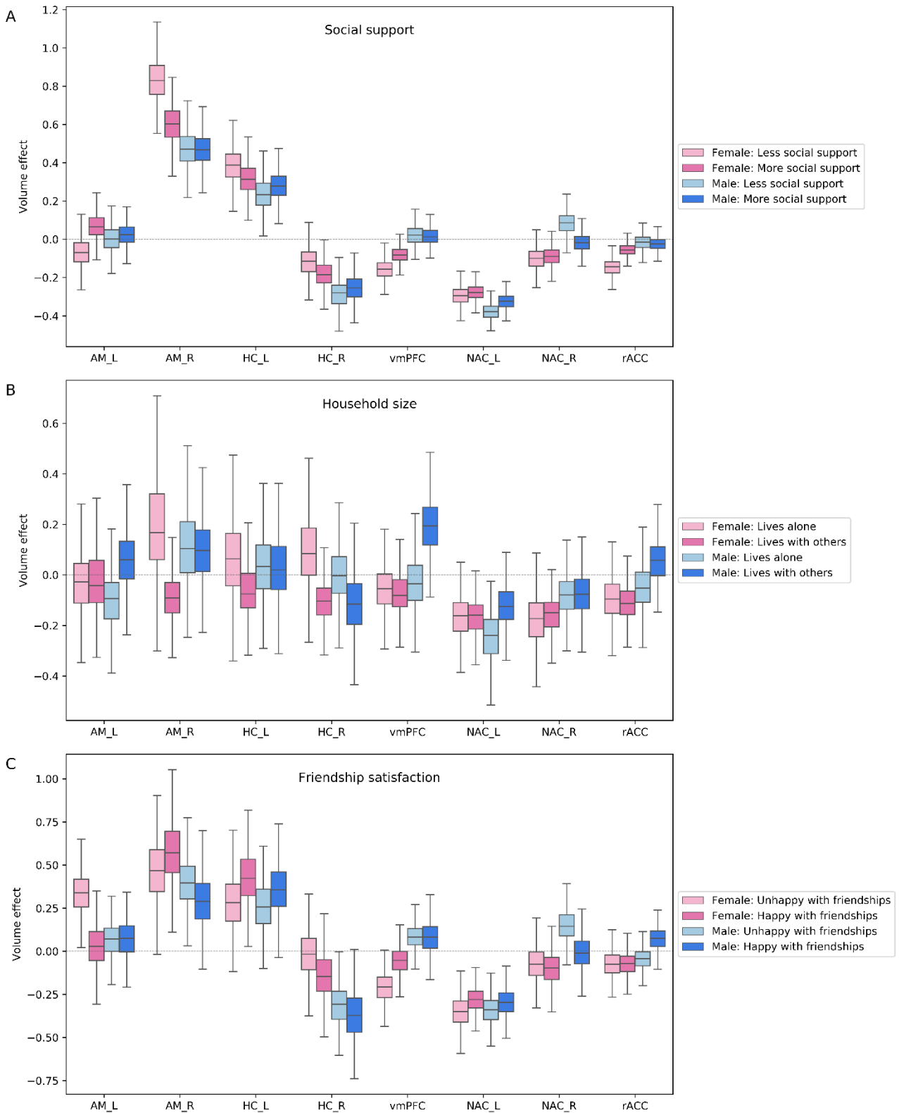
Figure 3. Population volume effects in the limbic network of the social brain. Boxplots depict four different subgroups in the context of (A) social support, (B) number of people living in the same household and (C) friendship satisfaction. (A) large volume effects were observed in the amygdala (AM), ventromedial prefrontal cortex (vmPFC) and rostral anterior cingulate cortex (rACC) in women and in the right nucleus accumbens (NAC_R) in men with less social support. (B) Volume effects were incongruent in the right amygdala (AM_R) in women and in the ventromedial prefrontal cortex (vmPFC) in men living with others. (C) Volume effects were uncovered in the left amygdala (AM_L) and ventromedial prefrontal cortex (vmPFC) in women and in the right nucleus
