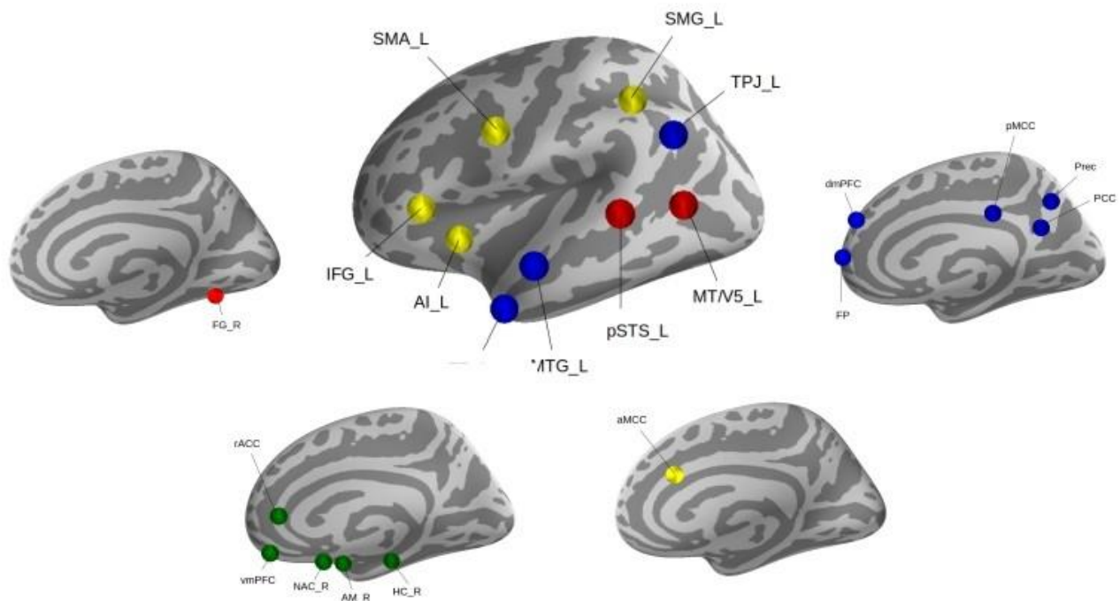
Figure 1. Social brain atlas. Thirty-six brain regions were previously automatically separated into i) visual-sensory network (red), ii) limbic network (green), iii) intermediate-level network (yellow),
