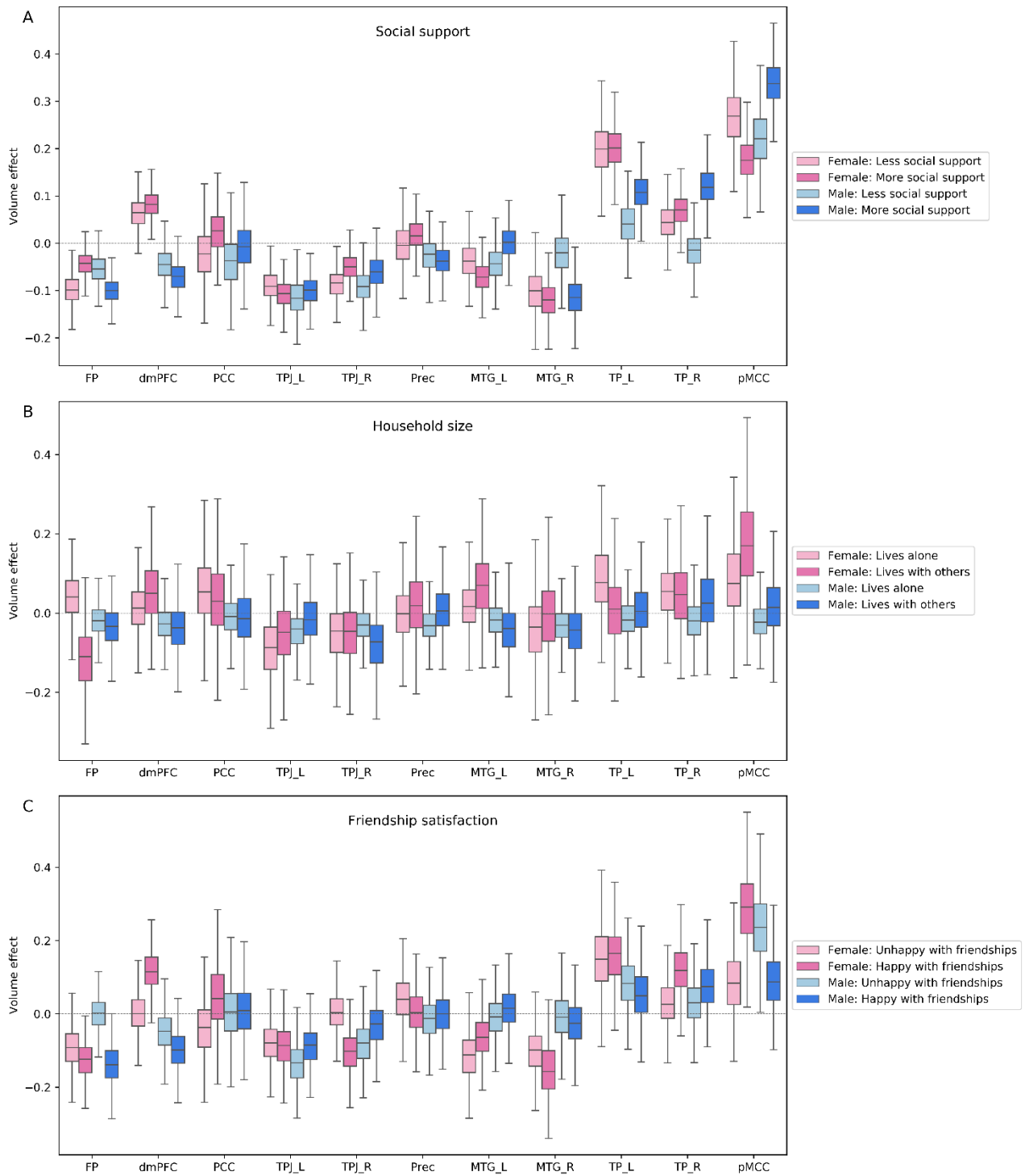
Figure 5. Population volume effects in the higher-associative network of the social brain. Boxplots depict four different subgroups in the context of (A) social support, (B) number of people living in the same household and (C) friendship satisfaction. (A) Volume effects were revealed in the frontal pole (FP), right middle temporal gyrus (MTG_R), right and left temporal pole (TP_R, TP_L) and posterior mid-cingulate cortex (pMCC) in men with more social support and in the frontal pole (FP) and posterior mid-cingulate cortex (pMCC) in women with less social support. (B) Household size analysis showed a volume effect in the frontal pole (FP) for women living with others. (C) The volume effects were incongruent in the dorsomedial prefrontal cortex (dmPFC), right temporoparietal junction (TPJ_R) and posterior mid-cingulate cortex (pMCC) in women with happy friendships and in posterior mid-cingulate cortex (pMCC) for men with unhappy and in frontal pole
