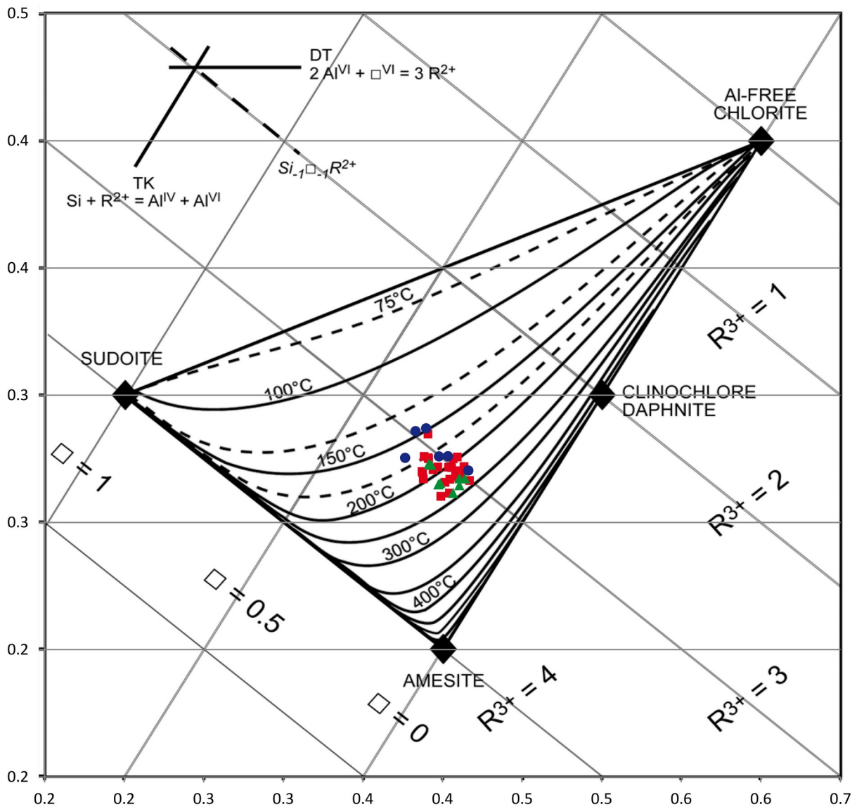
Fig. 14. Si vs R^{2+} diagram (Bourdelle & Cathelineau, 2015) for Fe-chlorites in Oklo-Okélobondo (green triangles), Bangombé (red squares) and Mikouloungou (blue dots) samples.
