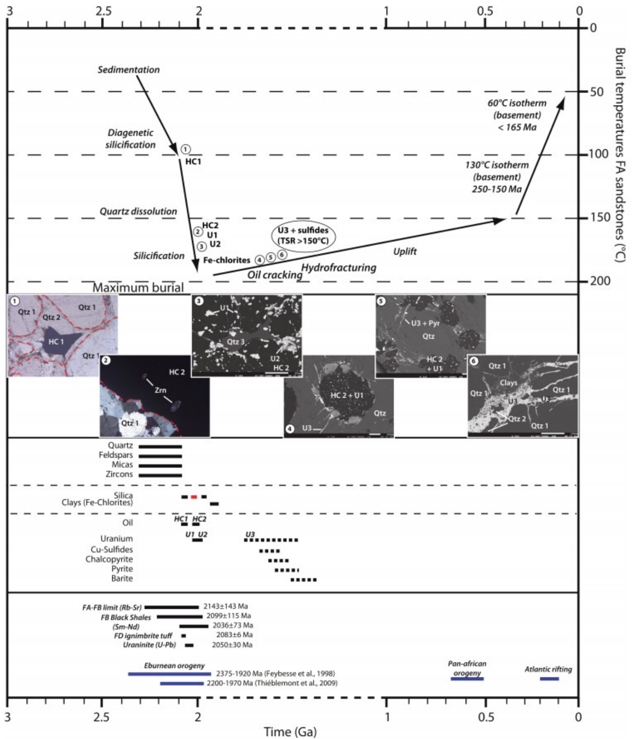
Fig. 15. Summary diagram of oil migration and uranium mineralization in FA sandstones. Additional age data are summarized in Gauthier-Lafaye (2006). Orogeny ages are from Feybessse et al. , 1998 and Thiéblemont et al. , 2009. A complete list of previous data can be found in Mathieu (1999).
