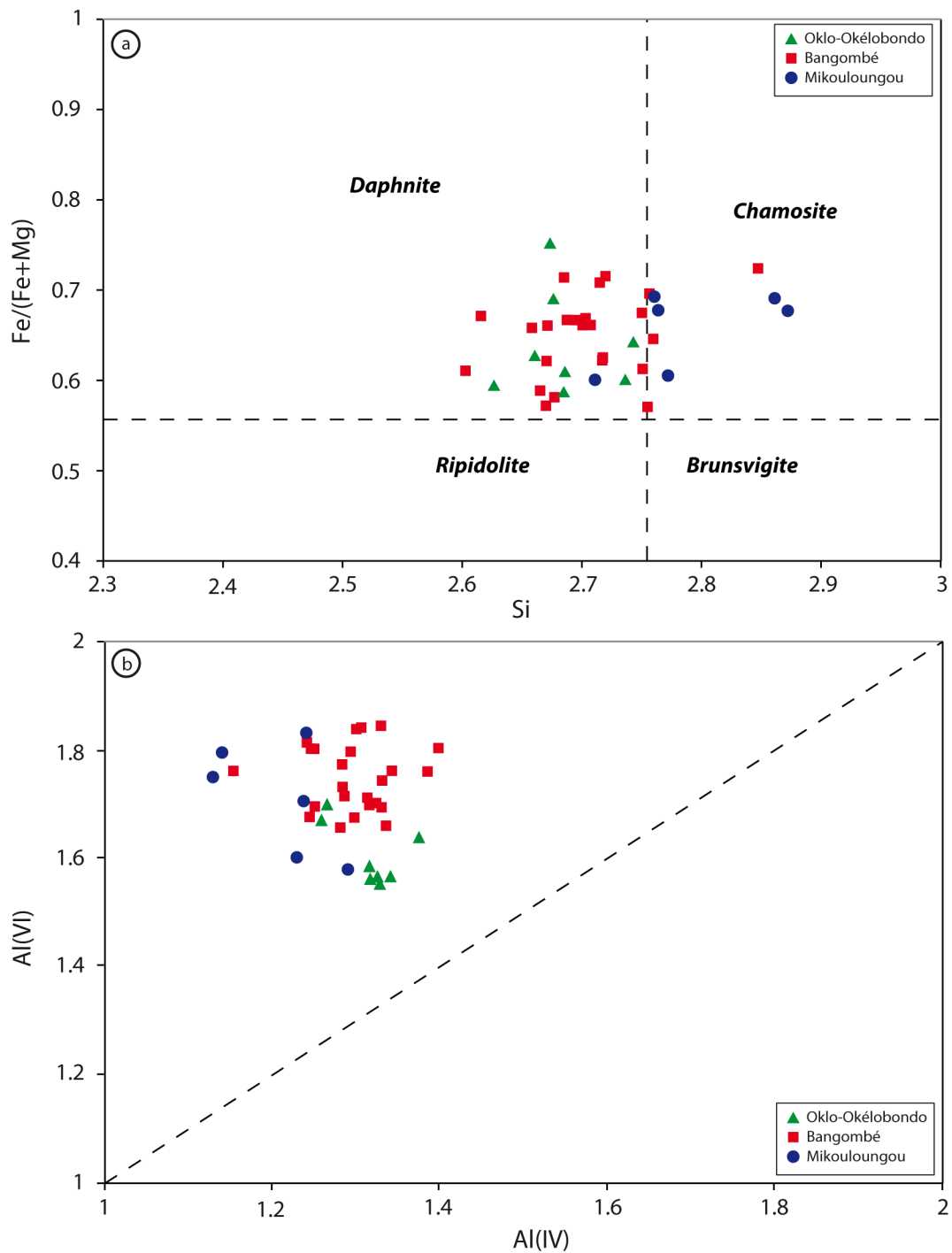
Fig. 13. Fe/(Fe+Mg) vs Si and Al(VI) vs Al(IV) diagrams for Fe-chlorites in Oklo-Okélobondo (green triangles), Bangombé (red squares) and Mikouloungou (blue dots) samples.
