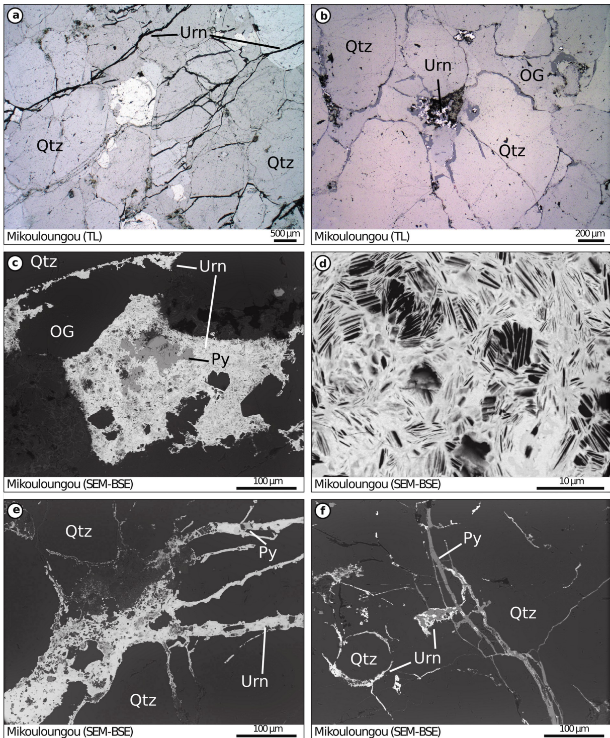
Fig. 8. Petrographic features of fractures in FA sandstones. a. Fracture network crosscutting detrital quartz (Qtz) and overgrowths (OG). b. Fractures and \text{UO}_2 precipitation at the boundary between detrital quartz and overgrowths. c. \text{UO}_2 precipitation on clays and at the boundary between detrital quartz and overgrowths. d. Detail of \text{UO}_2 and illites. e. Fractures filled by \text{UO}_2 and pyrite. f. Fractures filled by \text{UO}_2 and pyrite.
