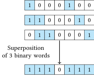
Fig. 1. Superposition of the binary words 1000100, 1100010 and 0110001.
