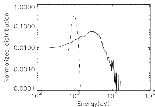
Figure 1: Energetic spectrum of solar wind protons after reflection on the Martian bow shock (continuous curve) compared to their initial spectrum.
