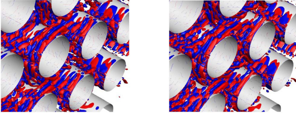
(a) (b) Figure 7: \omega_z vorticity iso-surfaces for the DDES- k - \omega -OES model (b) within a time interval of 10 dimensionless time-units.
