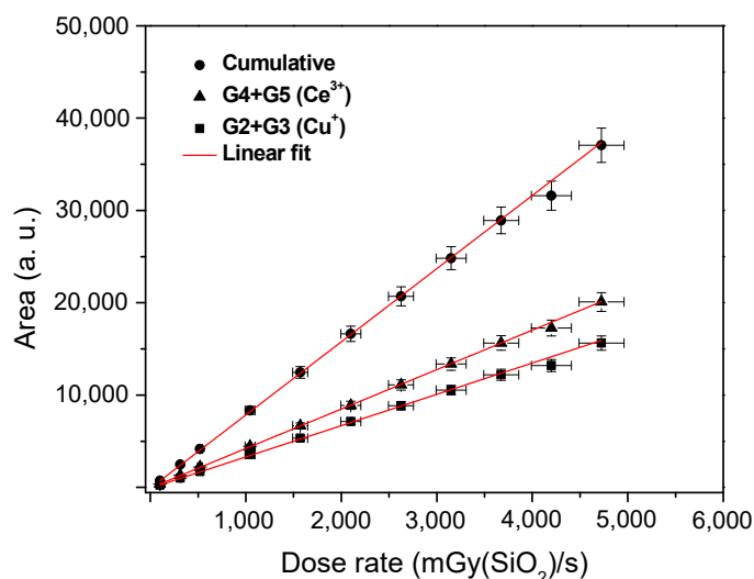
Figure 9. Integrated intensities of the whole RL spectrum and of Gaussian sub-bands related to \text{Cu}^+ ( \text{G2} + \text{G3} ) and \text{Ce}^{3+} ( \text{G4} + \text{G5} ) ions plotted versus the dose rate.
